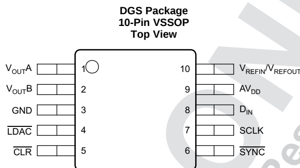
Pin Functions
