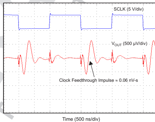
图 48. Clock Feedthrough 500 kHz, Mid-Scale
