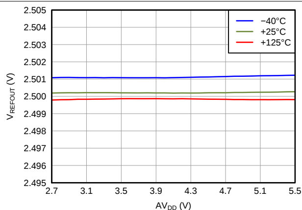
图 7. Internal Reference Voltage vs Supply Voltage
