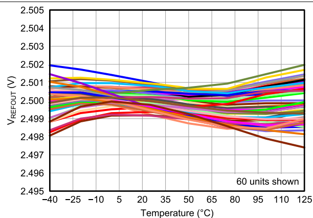
图 2. Internal Reference Voltage vs Temperature
