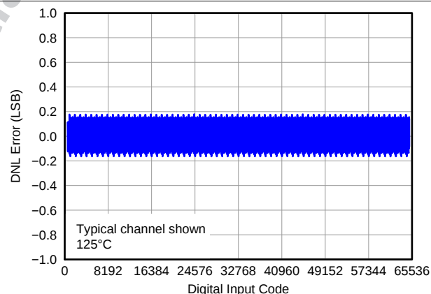
图 60. Differential Linearity Error vs Digital Input Code ( 125^\circ\text{C} )
