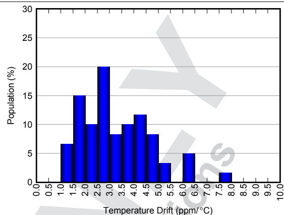
图 3. Internal Reference Voltage Temperature Drift Histogram
