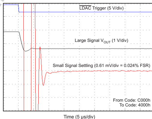
图 78. Half-Scale Settling Time: Falling Edge
