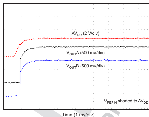
图 86. Power-On Glitch Reset to Mid-Scale
