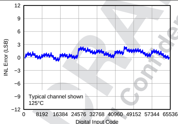
图 59. Linearity Error vs Digital Input Code ( 125^\circ\text{C} )
