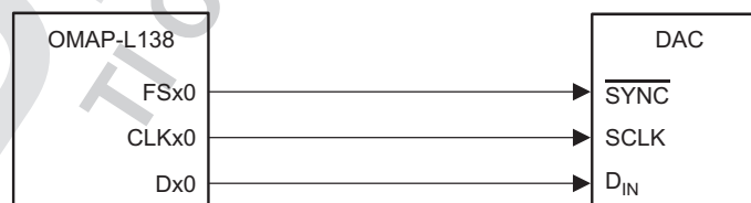
图 102. DAC756x-Q1, DAC816x-Q1, or DAC856x-Q1 Device to OMAP-L1x Processor
