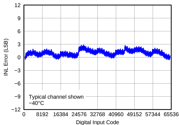
图 55. Linearity Error vs Digital Input Code ( -40^\circ\text{C} )
