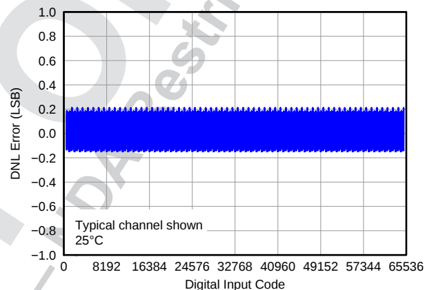
图 58. Differential Linearity Error vs Digital Input Code ( 25^\circ\text{C} )
