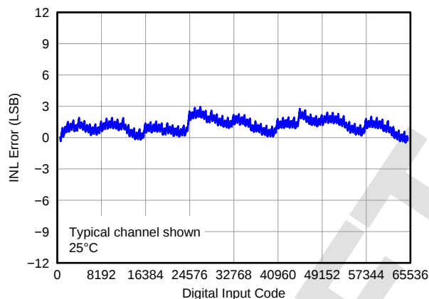
图 57. Linearity Error vs Digital Input Code ( 25^\circ\text{C} )
