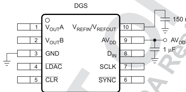
图 94. Typical Connection for Operating the DAC756x-Q1, DAC816x-Q1, and DAC856x-Q1 Internal Reference
