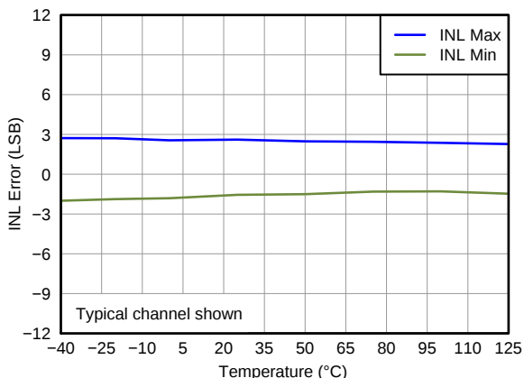
图 61. Linearity Error vs Temperature
