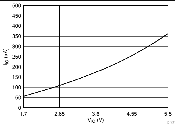
图 7-23. Supply Current ( I_{LO} ) vs Supply Voltage
