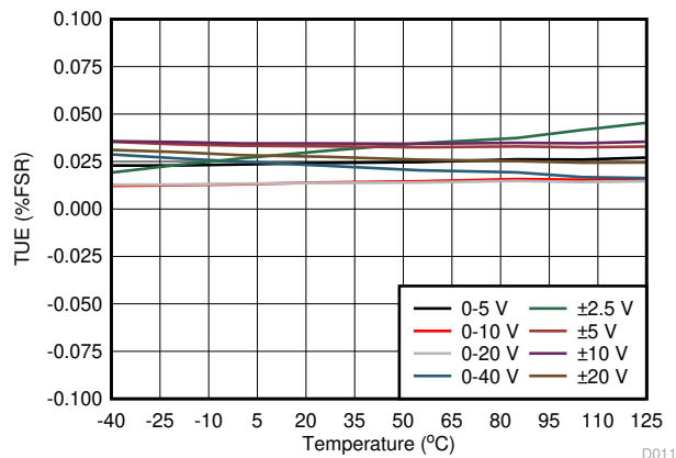
图 7-13. Total Unadjusted Error vs Temperature
