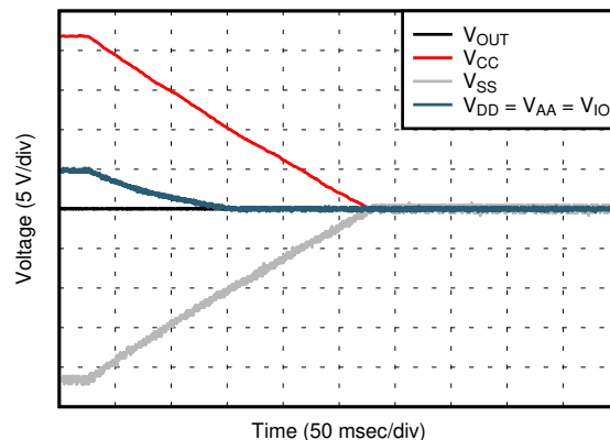
图 7-36. Power-Down Response
