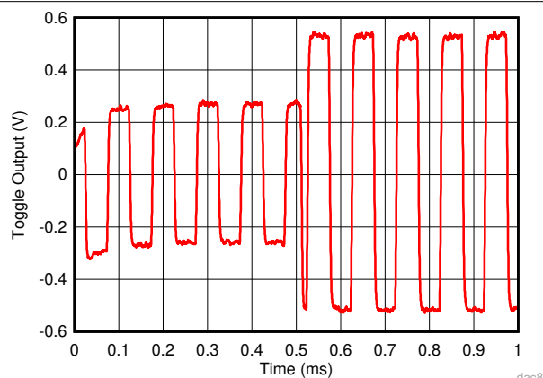
图 9-2. Toggle AC Amplitude Transition
