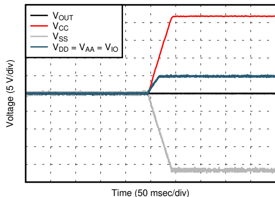
图 7-35. Power-Up Response
