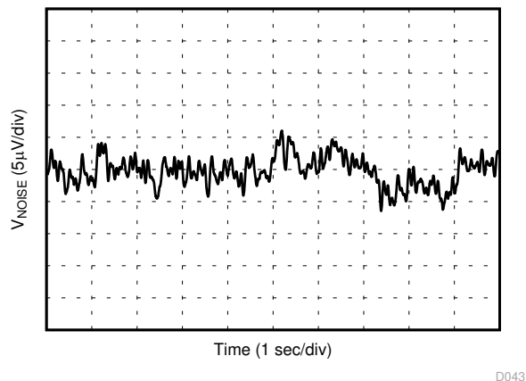
图 7-45. Internal Reference Noise
