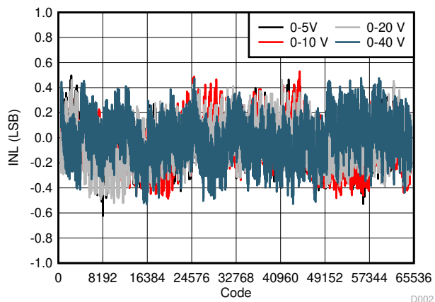
图 7-4. Integral Linearity Error vs Digital Input Code (Unipolar Outputs)
