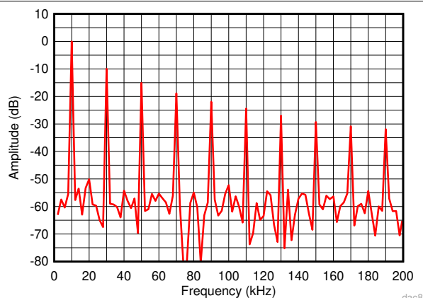
图 9-3. Frequency Spectrum of Toggle Output
