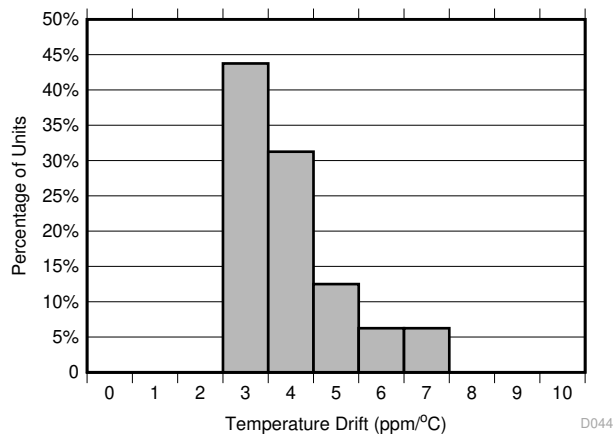
图 7-46. Internal Reference Temperature Drift Histogram
