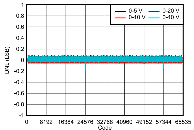
图 7-6. DAC81404 DNL vs Digital Input Code (Unipolar Outputs)
