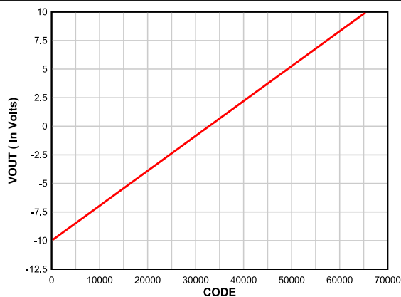
图 9-2. DAC Code Sweep From -10 V to +10 V
