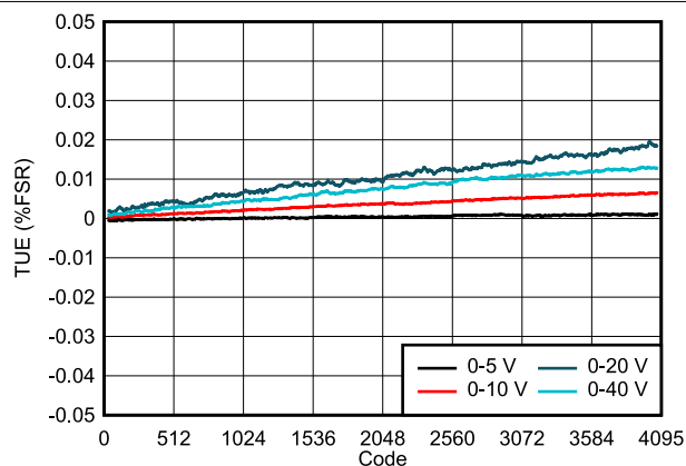
图 7-14. DAC61404 TUE vs Digital Input Code (Unipolar Outputs)
