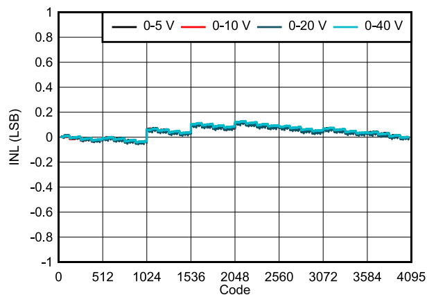
图 7-10. DAC61404 INL vs Digital Input Code (Unipolar Outputs)
