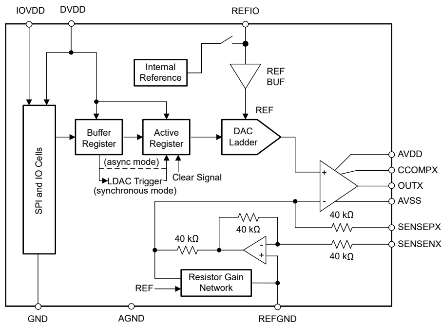
图 8-1. Device Architecture
