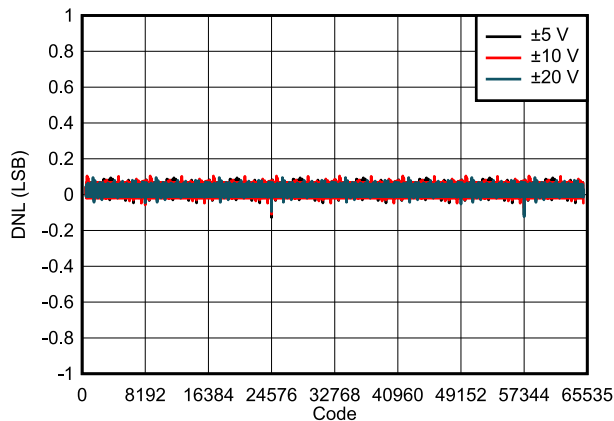
图 7-5. DAC81404 DNL vs Digital Input Code (Bipolar Outputs)
