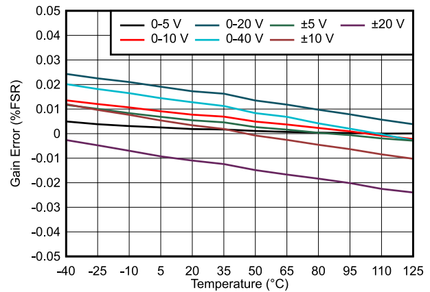
图 7-24. Gain Error vs Temperature
