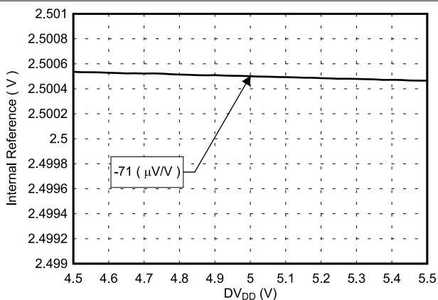
图 7-44. Internal Reference Voltage vs Supply Voltage
