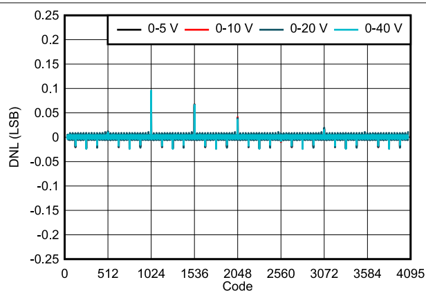
图 7-12. DAC61404 DNL vs Digital Input Code (Unipolar Outputs)
