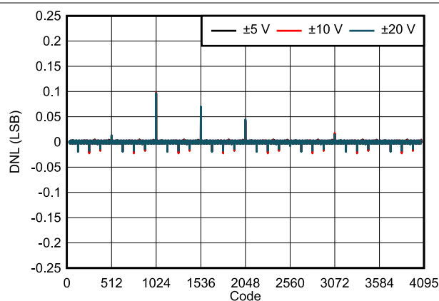
图 7-11. DAC61404 DNL vs Digital Input Code (Bipolar Outputs)
