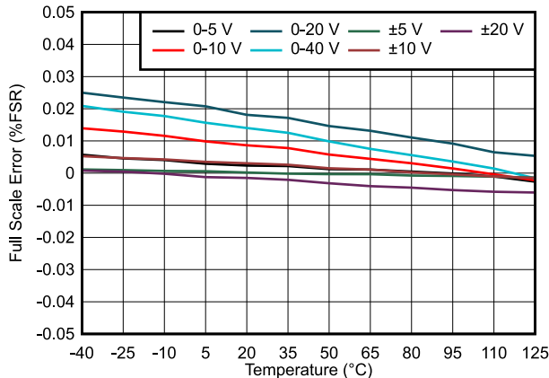
图 7-25. Full-Scale Error vs Temperature
