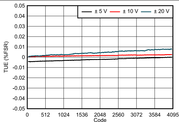
图 7-13. DAC61404 TUE vs Digital Input Code (Bipolar Outputs)
