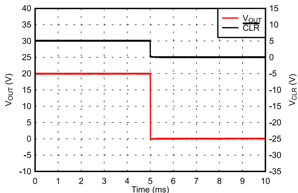
图 7-40. Clear Command Response
