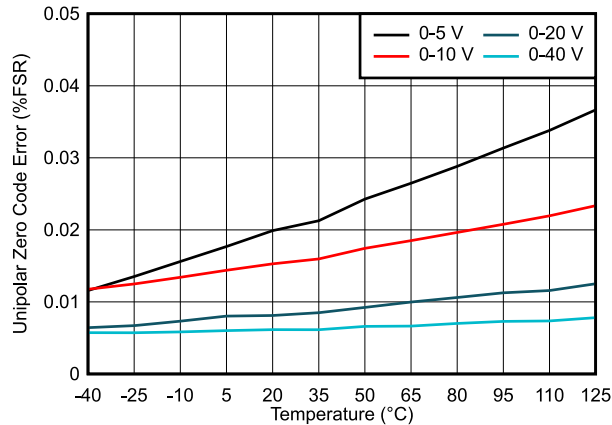
图 7-21. Unipolar Zero Code Error vs Temperature
