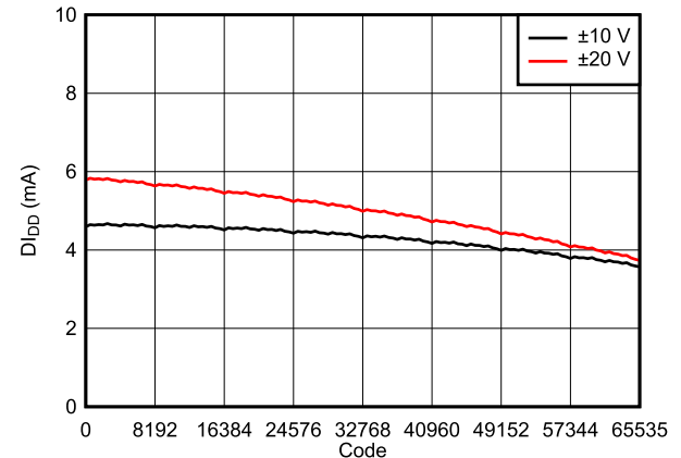
图 7-26. Supply Current ( DI_{DD} ) vs Digital Input Code
