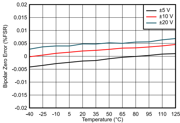
图 7-23. Bipolar Zero Error vs Temperature
