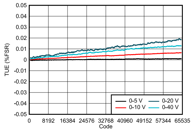
图 7-8. DAC81404 TUE vs Digital Input Code (Unipolar Outputs)
