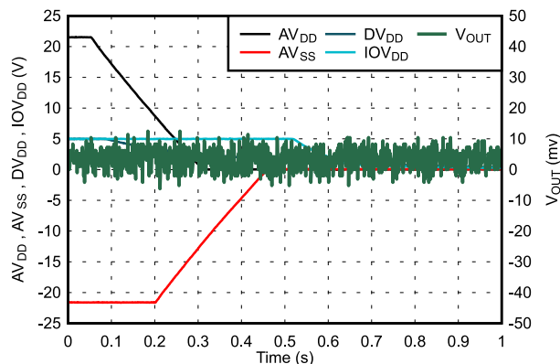
图 7-39. Power-Down Response
