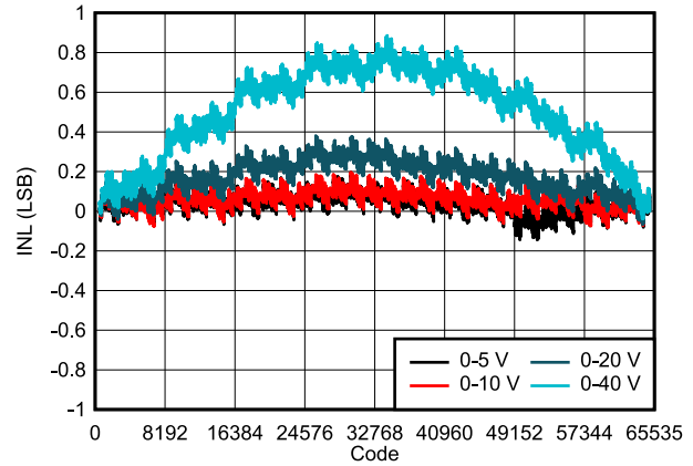
图 7-4. DAC81404 INL vs Digital Input Code (Unipolar Outputs)
