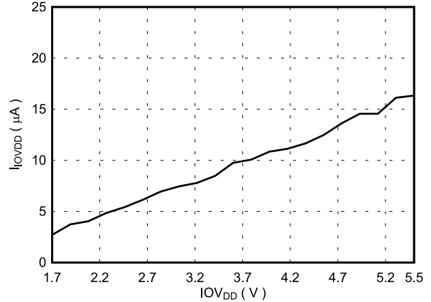
图 7-28. Supply Current ( I_{IOVDD} ) vs Supply Voltage
