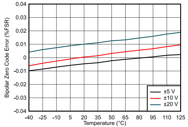
图 7-22. Bipolar Zero Code Error vs Temperature
