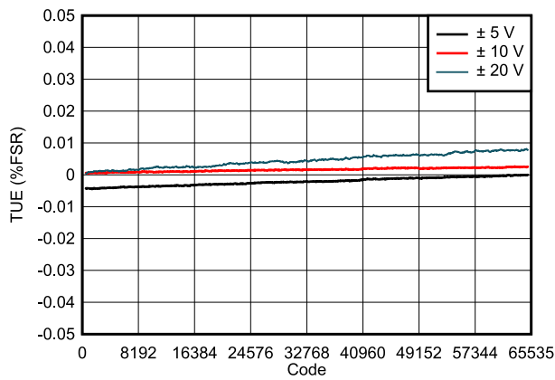
图 7-7. DAC81404 TUE vs Digital Input Code (Bipolar Outputs)
