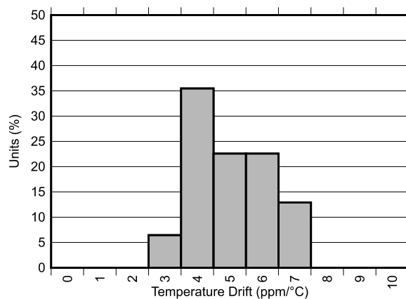
图 7-48. Internal Reference Temperature Drift Histogram
