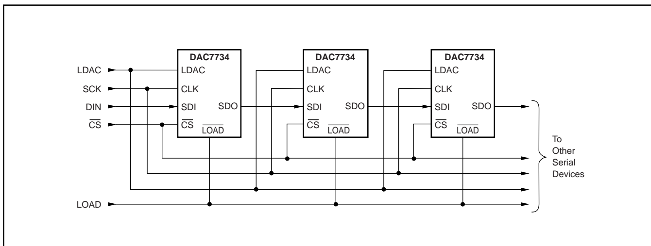
FIGURE 11. Daisy-Chaining DAC7734.
