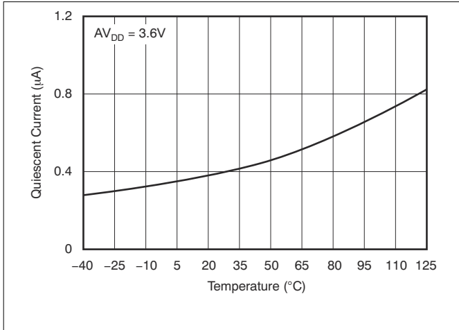
图 7-39. Power-Down Current vs Temperature
