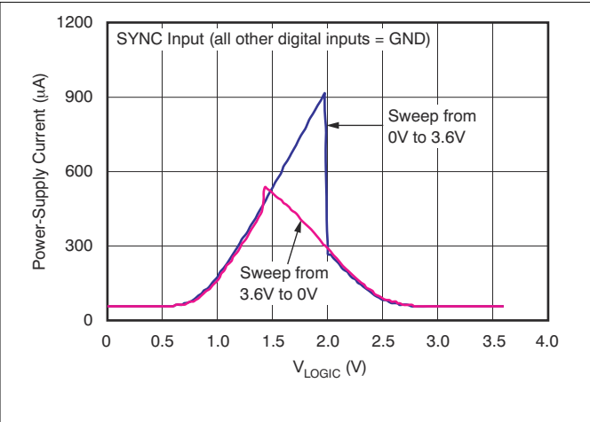
图 7-40. Power-Supply Current vs Logic Input Voltage
