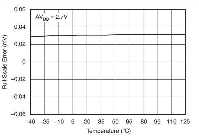
图 7-55. Full-Scale Error vs Temperature
