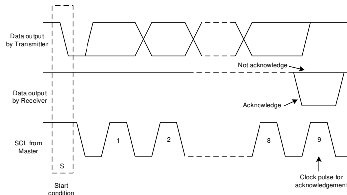
图 59. Acknowledge and Not Acknowledge on the I 2 C Bus
