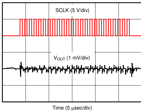
DAC code at midscale, external reference = 2.5 V, SCLK = 1 MHz, REF-DIV = 0 and BUFF-GAIN = 0
