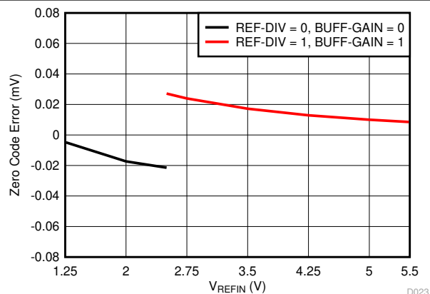
图 7-23. Zero Code Error vs Reference Voltage
