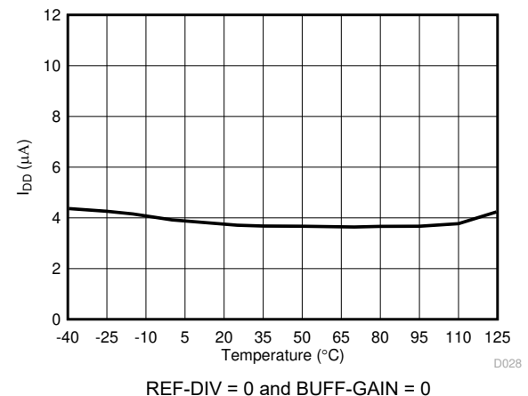
图 7-30. Power Down Current vs Temperature
