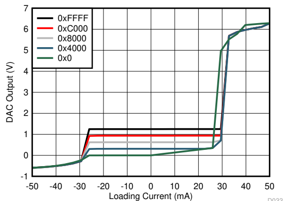
图 7-33. Source and Sink Capability
