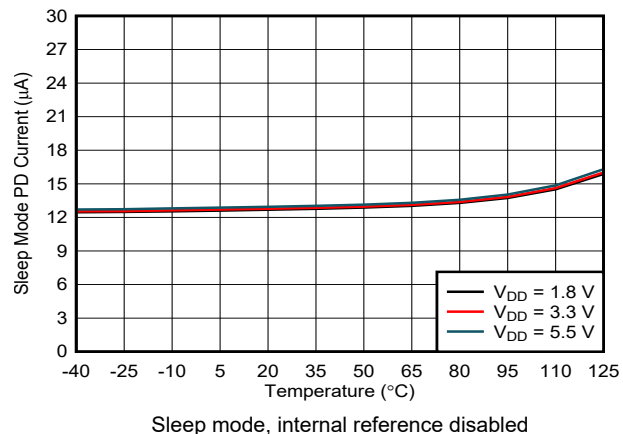
图 6-56. Power-Down Current vs Temperature
