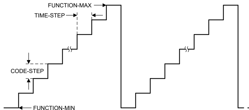
图 7-13. Sawtooth Waveform
