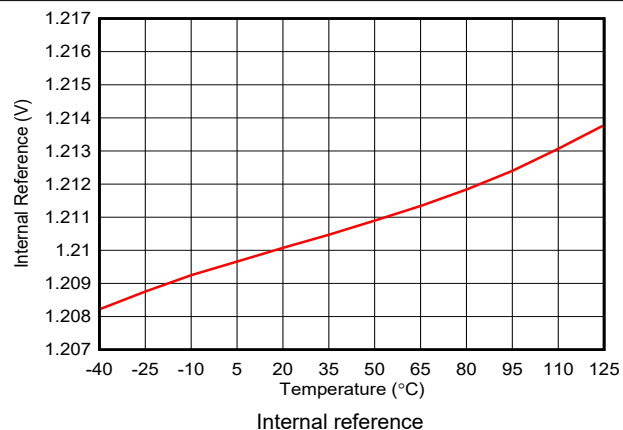
图 6-54. Internal Reference vs Temperature
