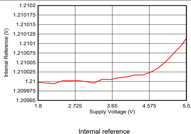
图 6-55. Internal Reference vs Supply Voltage
