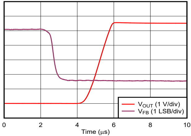
图 6-51. Comparator Response Time: Low-to-High Transition
