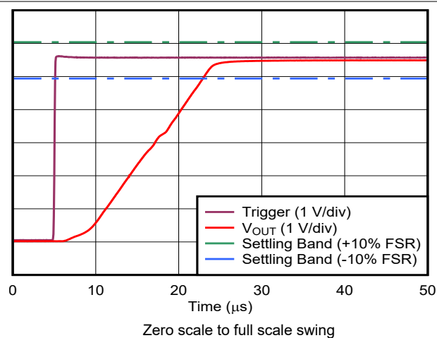
图 6-21. Voltage Output Setting Time: Rising Edge
