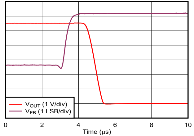
图 6-52. Comparator Response Time: High-to-Low Transition
