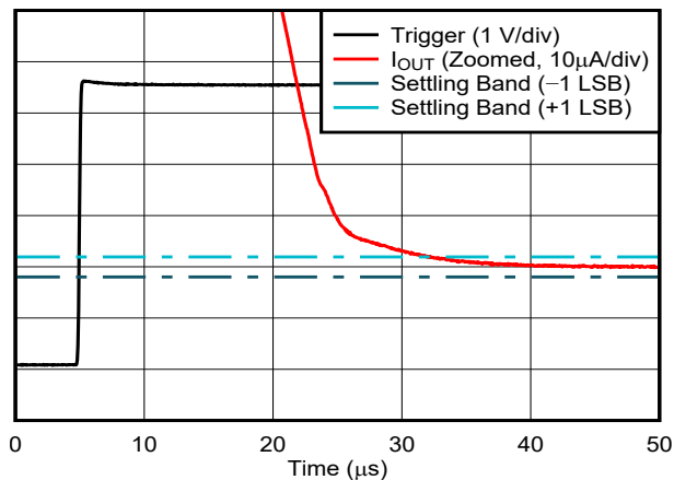
图 6-43. Current Output Setting Time, Falling Edge
