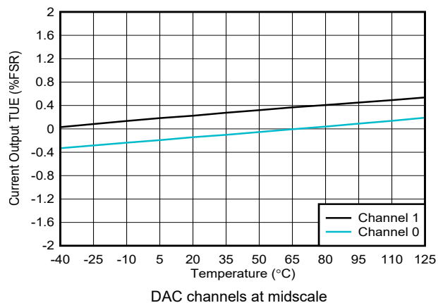
图 6-37. Current Output TUE vs Temperature
