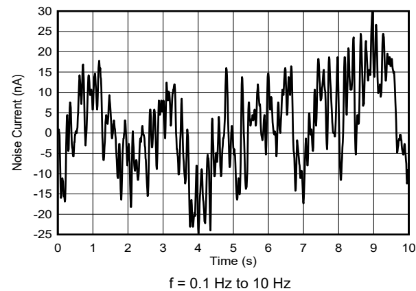
图 6-47. Current Output Flicker Noise
