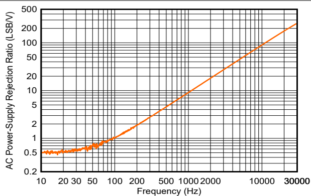
图 6-48. Current Output AC PSRR vs Frequency
