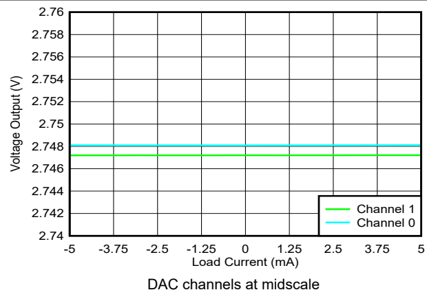
图 6-18. Voltage Output vs Load Current
