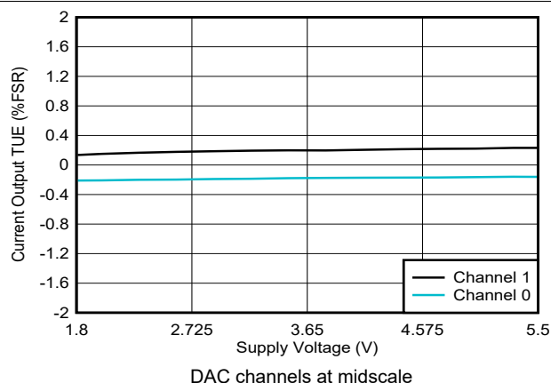
图 6-38. Current Output TUE vs Supply Voltage
