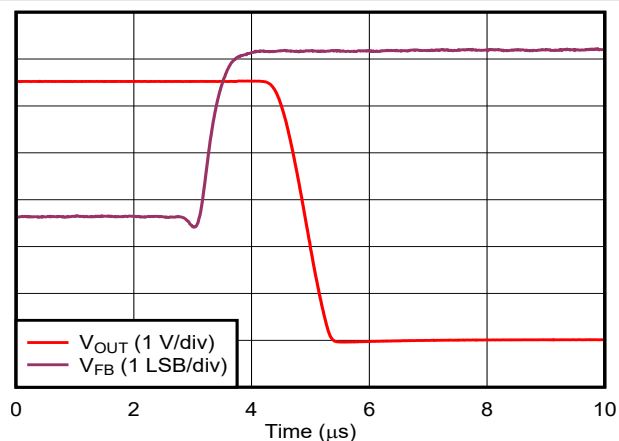
图 6-50. Comparator Response Time: High-to-Low Transition
