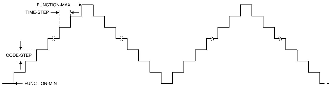
图 7-12. Triangle Waveform
