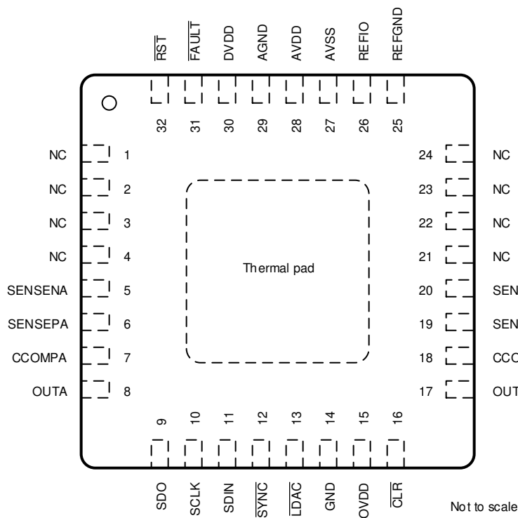
图 6-1. RHB (32-pin VQFN) Package, Top View
