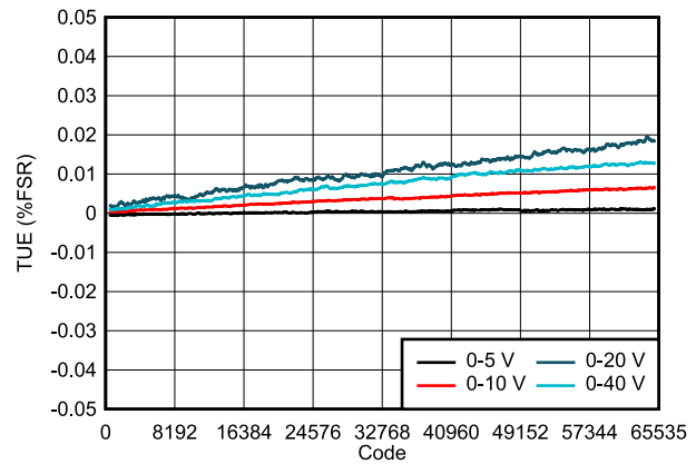
图 7-8. DAC81402 TUE vs Digital Input Code (Unipolar Outputs)
