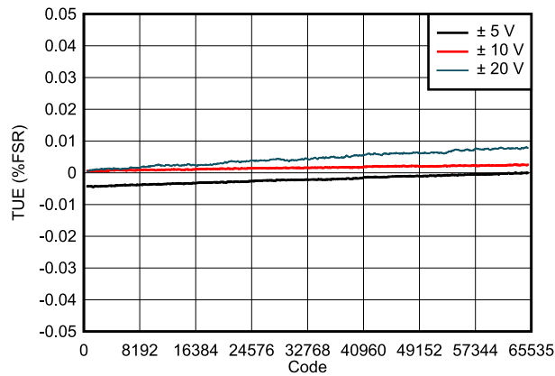
图 7-7. DAC81402 TUE vs Digital Input Code (Bipolar Outputs)
