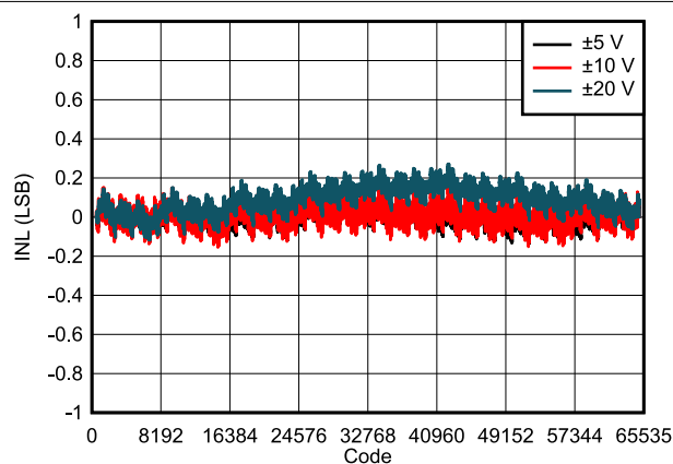
图 7-3. DAC81402 INL vs Digital Input Code (Bipolar Outputs)
