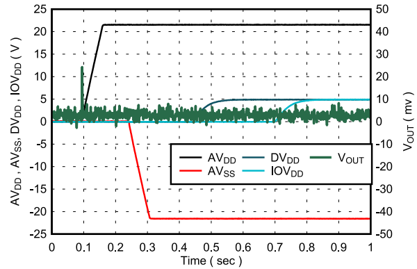
图 7-38. Power-Up Response
