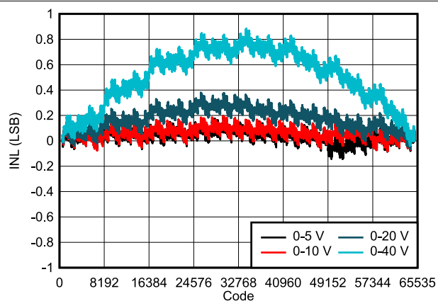
图 7-4. DAC81402 INL vs Digital Input Code (Unipolar Outputs)
