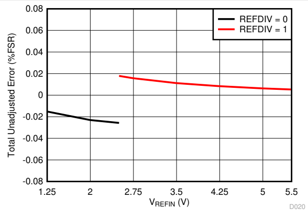
图 7-22. Total Unadjusted Error vs Reference Voltage
