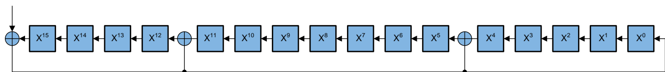
Figure 44. CRC CCITT 16
