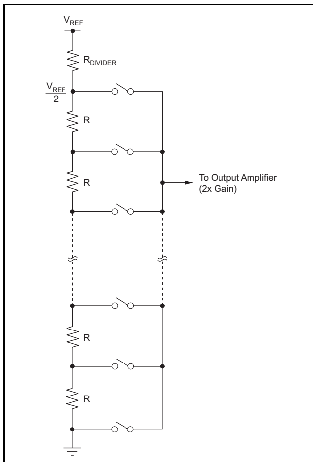
Figure 112. Resistor String
