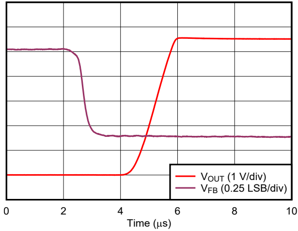
Comparator output in push-pull mode
