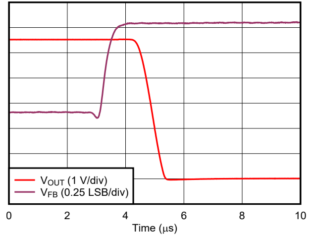
Comparator output in push-pull mode
