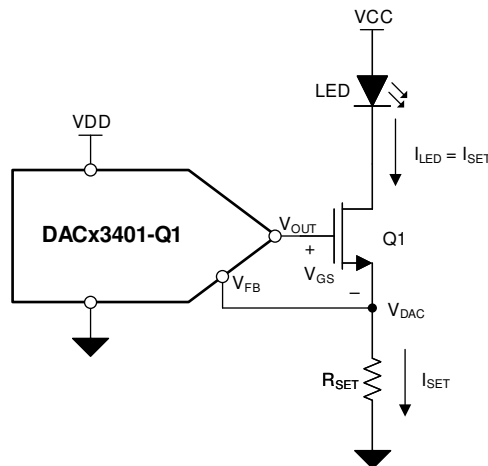
图 9-1. LED Biasing
