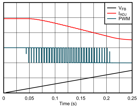
图 8-5. LED Thermal Foldback
