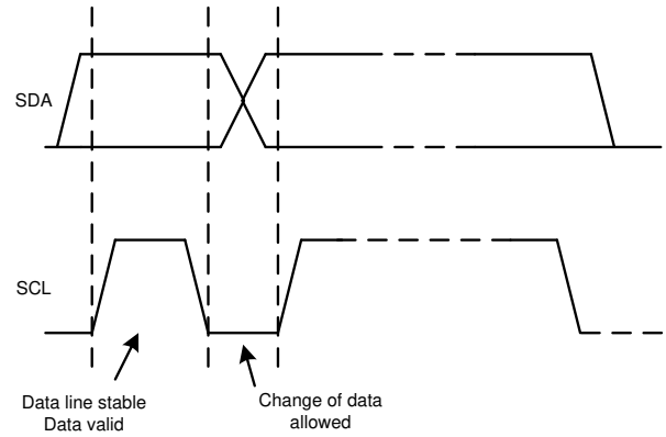
图 8-5. Bit Transfer on the I 2 C Bus
