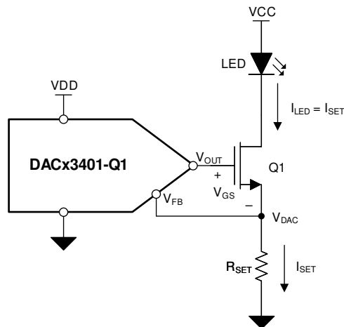
图 9-1. LED Biasing
