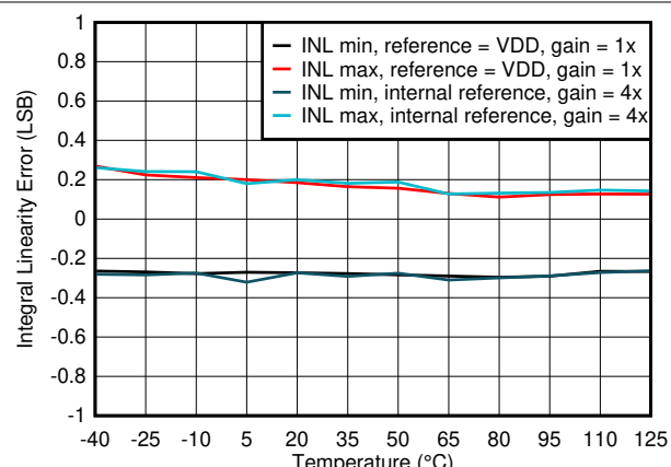
图 7-14. Integral Linearity Error vs Temperature
