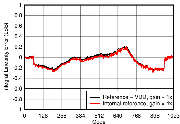
图 7-11. Integral Linearity Error vs Digital Input Code
