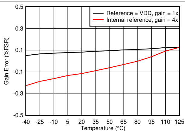
图 7-19. Gain Error vs Temperature
