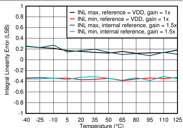
图 7-4. Integral Linearity Error vs Temperature
