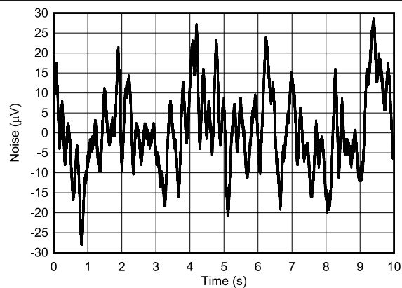
图 7-46. DAC Output Noise: 0.1 Hz to 10 Hz
