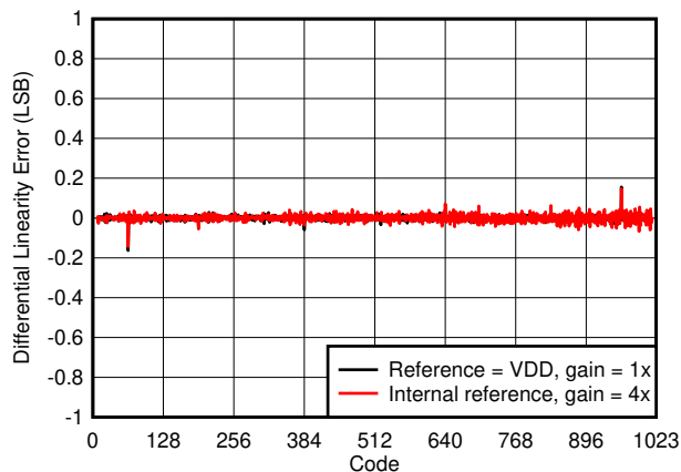
图 7-12. Differential Linearity Error vs Digital Input Code
