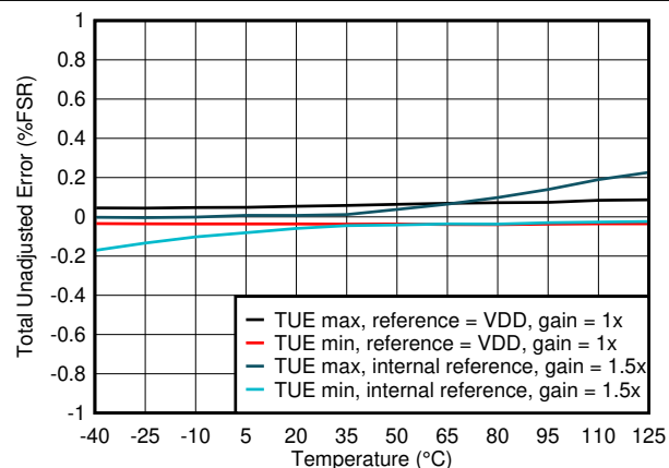
图 7-6. Total Unadjusted Error vs Temperature
