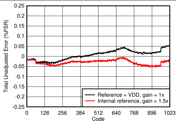
图 7-3. Total Unadjusted Error vs Digital Input Code
