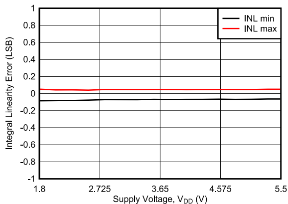
图 7-21. Integral Linearity Error vs Supply Voltage
