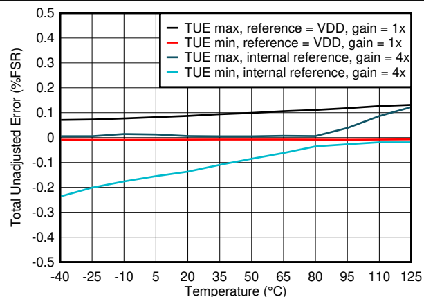
图 7-16. Total Unadjusted Error vs Temperature
