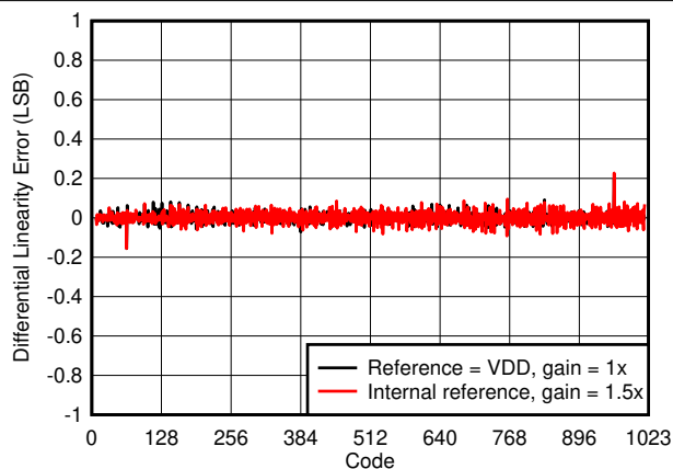
图 7-2. Differential Linearity Error vs Digital Input Code
