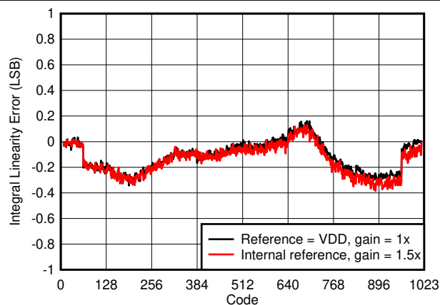
图 7-1. Integral Linearity Error vs Digital Input Code
