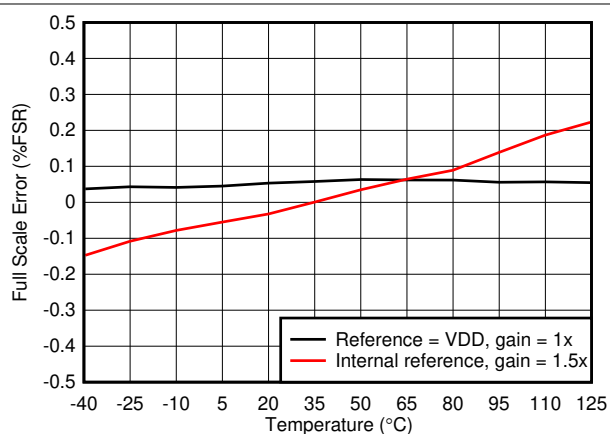
图 7-10. Full-Scale Error vs Temperature
