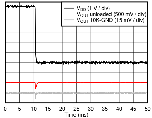
图 7-40. Power-off Glitch
