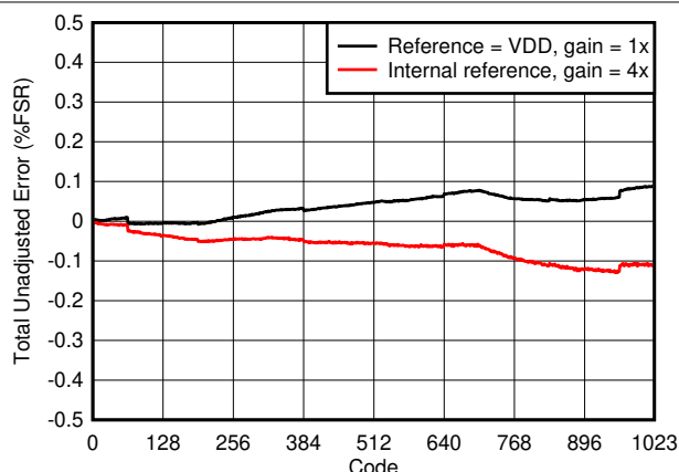
图 7-13. Total Unadjusted Error vs Digital Input Code
