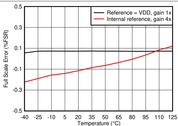
图 7-20. Full-Scale Error vs Temperature
