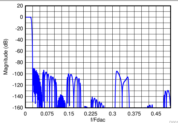
图 7-21. Composite Magnitude Response for 24x Interpolation
