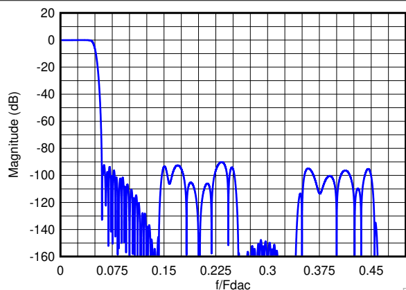
图 7-16. Composite Magnitude Response for 10x Interpolation
