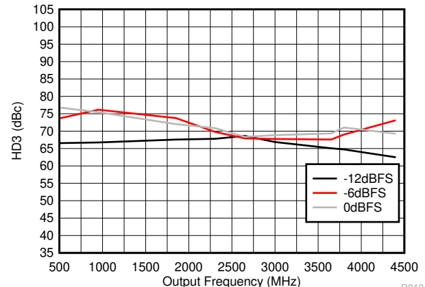
D013 DAC38RF80/90/84
