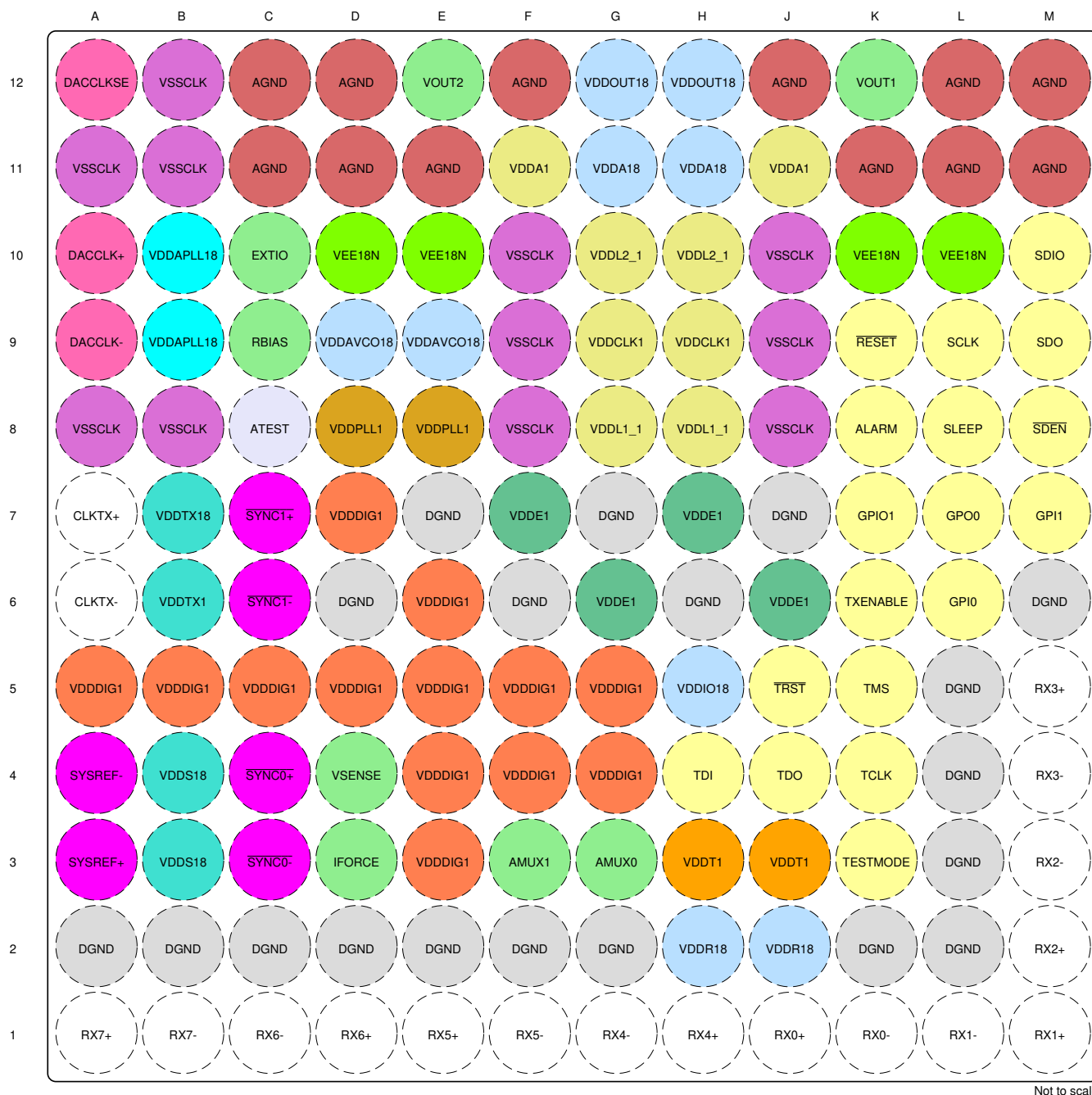
图 5-2. DAC38RF80, DAC38RF84, DAC38RF90 AAV Package 144-Pin (FCBGA) 144-Pin FCBGA Top View
