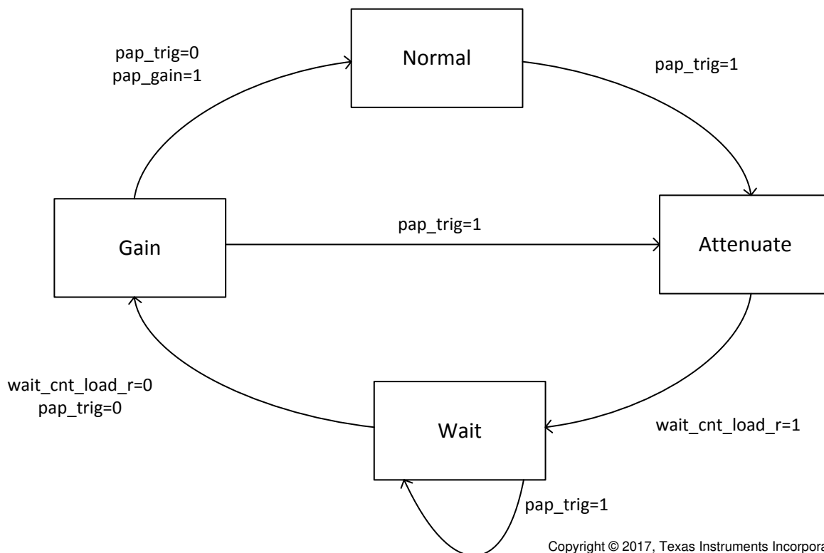
图 7-24. PAP Gain State Machine
