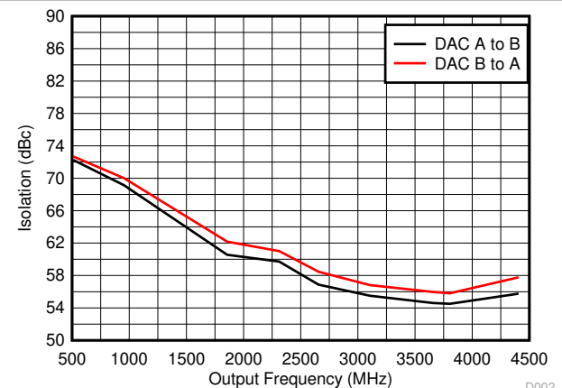
D002 DAC38RF80/90/84
