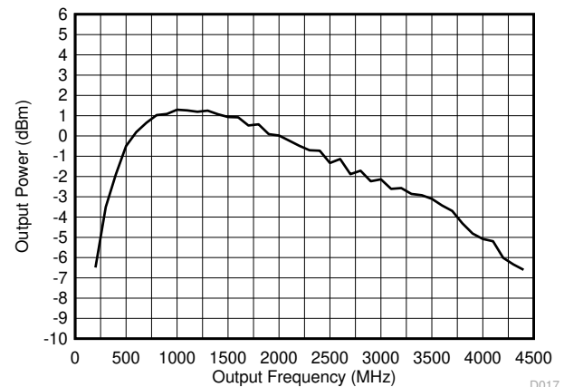
D017 DAC38RF80/90/84
