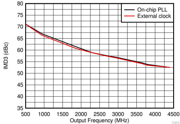
D016 DAC38RF83/93/85
