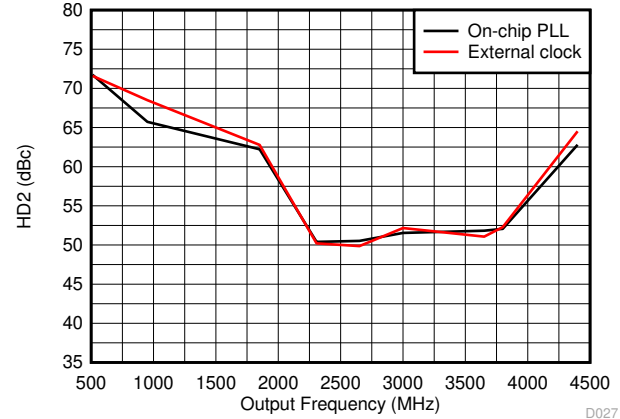
D027 DAC38RF80/90/84
