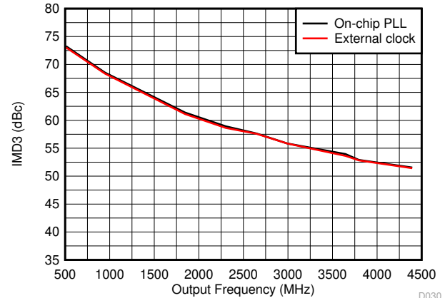
D030 DAC38RF80/90/84
