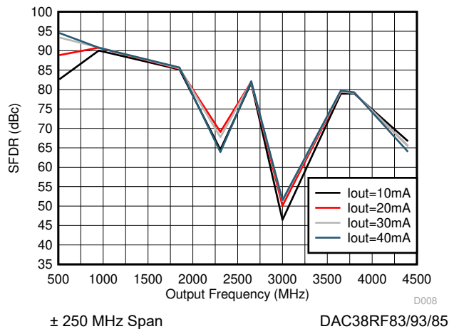
图 6-27. SFDR vs Output Frequency Over Output Current I_{\text{outFS}}
