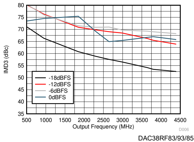
图 6-31. IMD3 vs Output Frequency Over Input Scale
