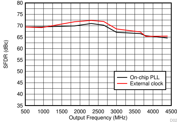
图 6-23. SFDR vs Output Frequency Over Clocking Option
