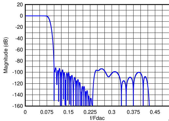
图 7-14. Composite Magnitude Response for 6x Interpolation
