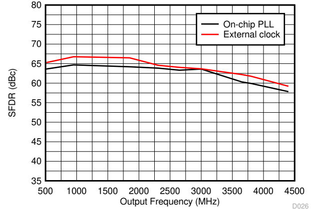
图 6-24. SFDR vs Output Frequency Over Clocking Option
