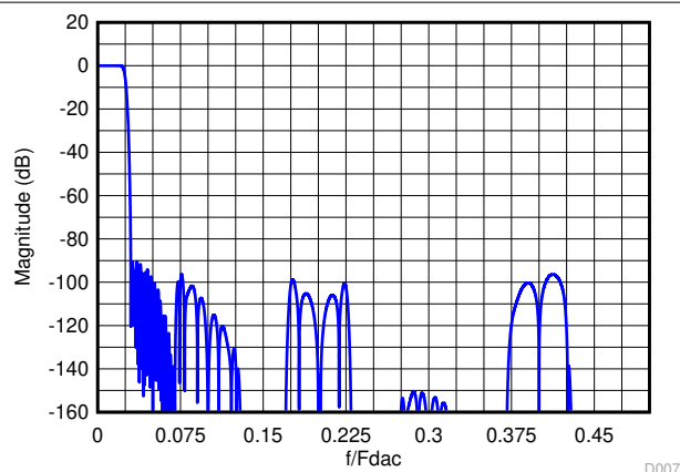
图 7-20. Composite Magnitude Response for 20x Interpolation
