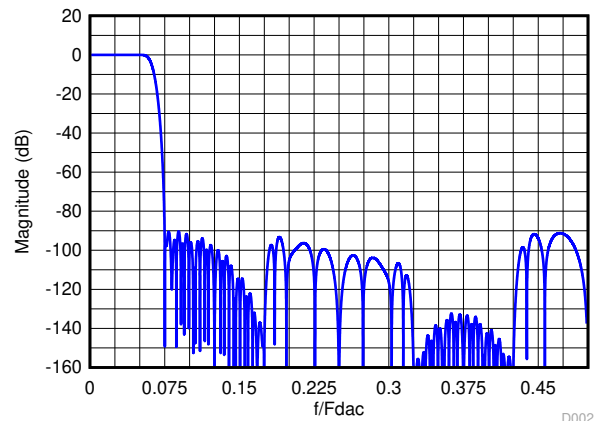
图 7-15. Composite Magnitude Response for 8x Interpolation
