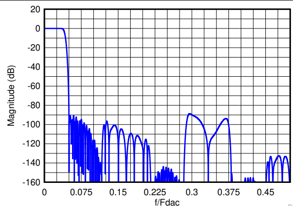
图 7-17. Composite Magnitude Response for 12x Interpolation
