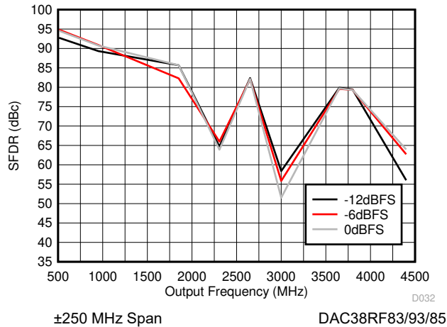
图 6-25. SFDR vs Output Frequency Over Input Scale
