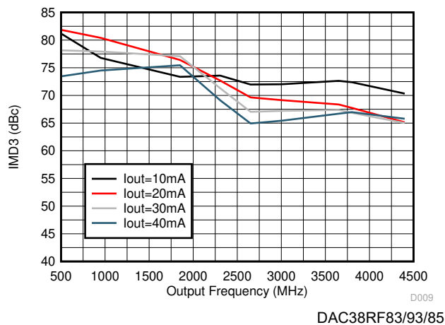
图 6-33. IMD3 vs Output Frequency Over Output Current I_{\text{outFS}}
