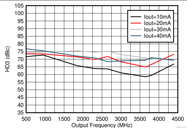
D014 DAC38RF80/90/84
