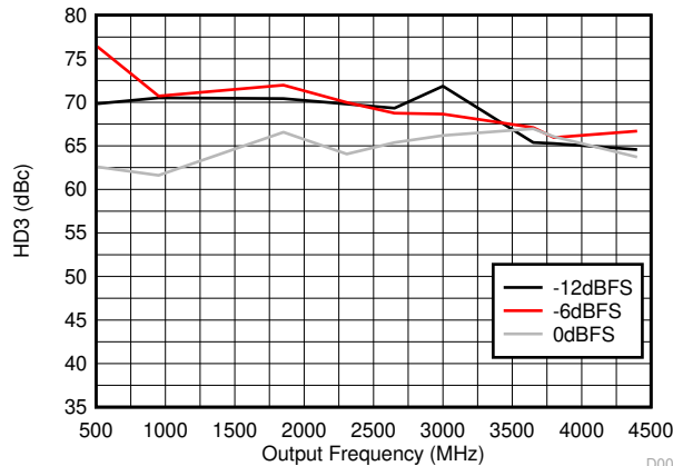
D004 DAC38RF83/93/85
