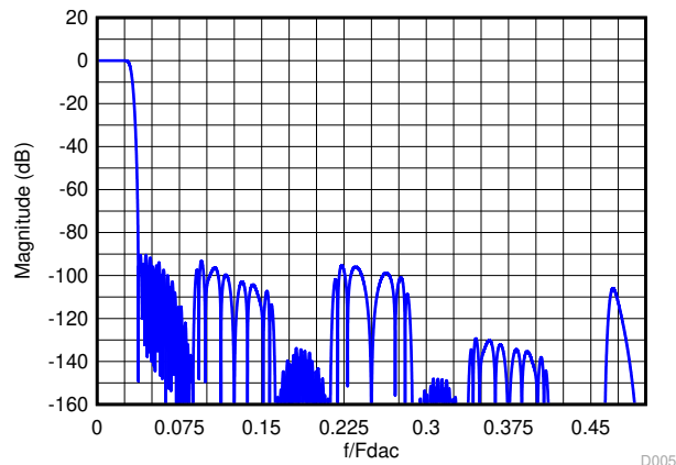
图 7-18. Composite Magnitude Response for 16x Interpolation
