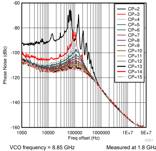
图 6-41. VCO1 Phase Noise vs Offset Frequency Over Charge pump current
