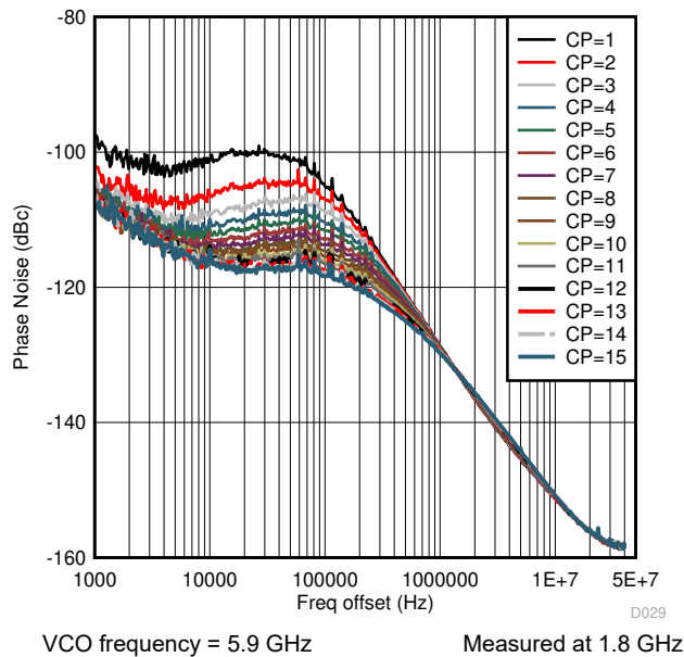
图 6-43. VCO0 Phase Noise vs Offset Frequency Over Charge Pump Current
