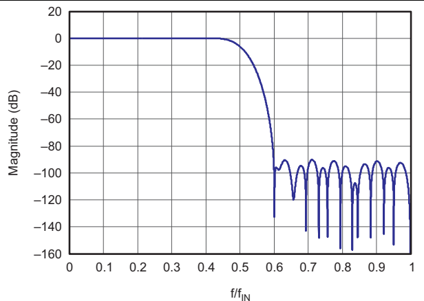
图 60. Magnitude Spectrum for FIR0
