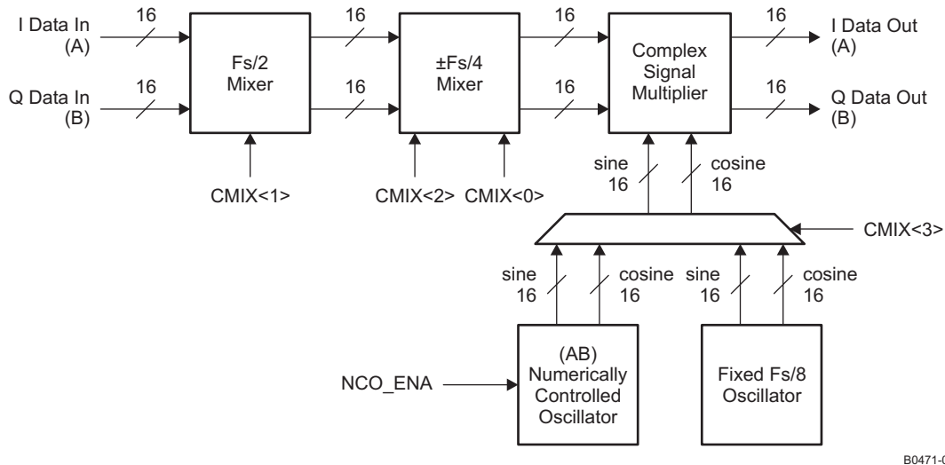
图 69. Path of Complex Signal Mixer
