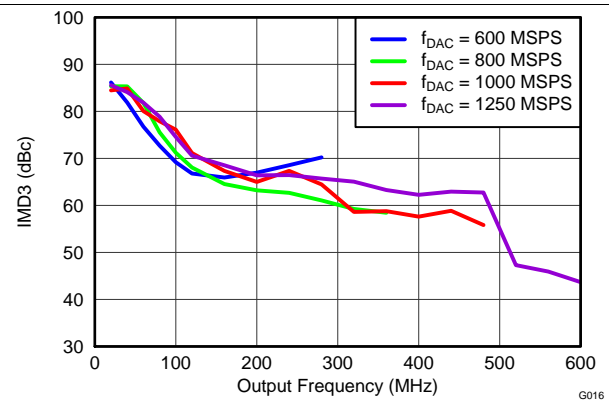
图 16. IMD3 vs Output Frequency Over f_{DAC}
