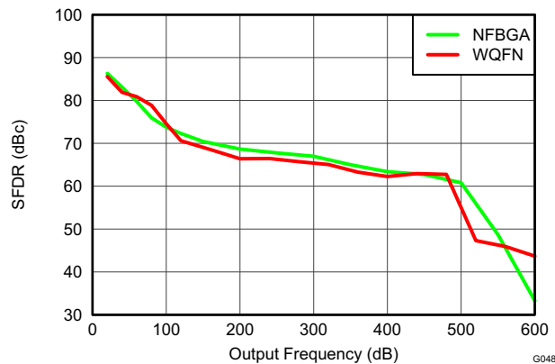
图 5-47. SFDR vs Output Frequency
