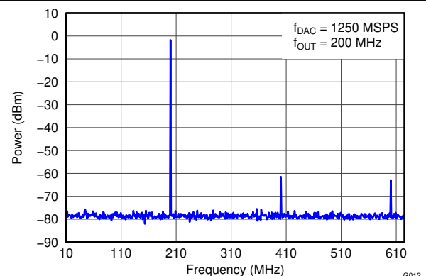
图 5-12. Single Tone Spectral Plot
