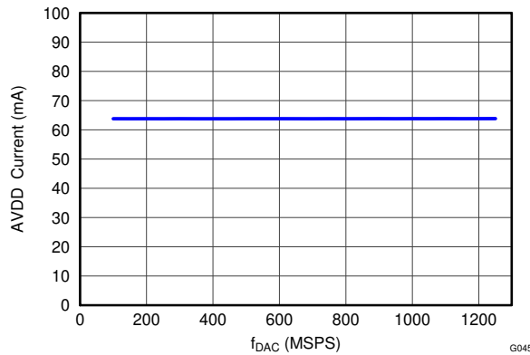
图 5-45. AVDD Current vs f_{DAC}
