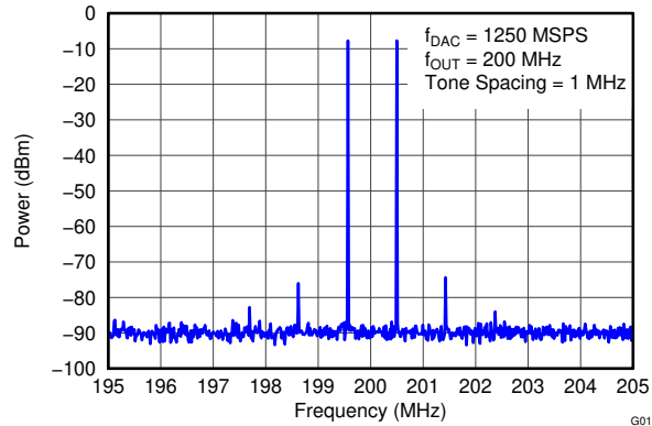
图 5-19. Two Tone Spectral Plot
