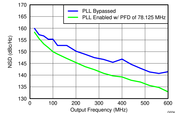
图 5-24. NSD vs Output Frequency Over Clocking Options
