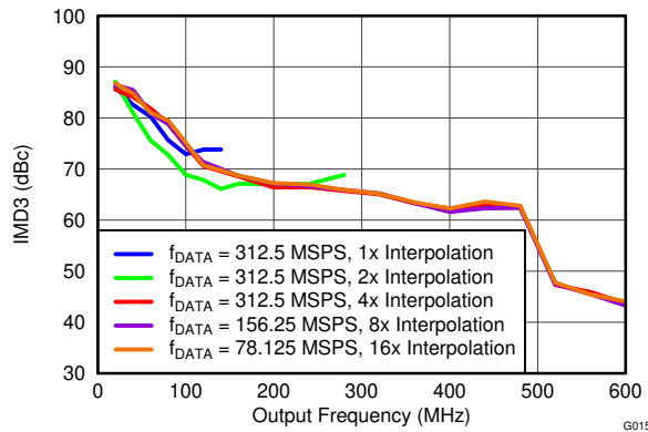
图 5-15. IMD3 vs Output Frequency Over Interpolation
