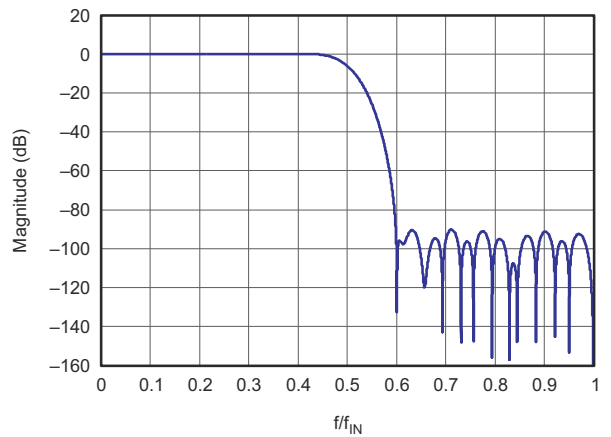
图 6-12. Magnitude Spectrum for FIR0
