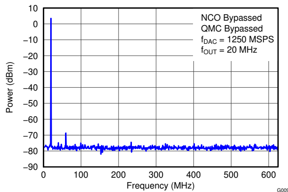
图 5-9. Single Tone Spectral Plot
