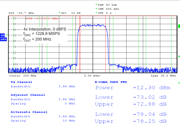
图 5-29. Single Carrier W-CDMA Test Model 1
