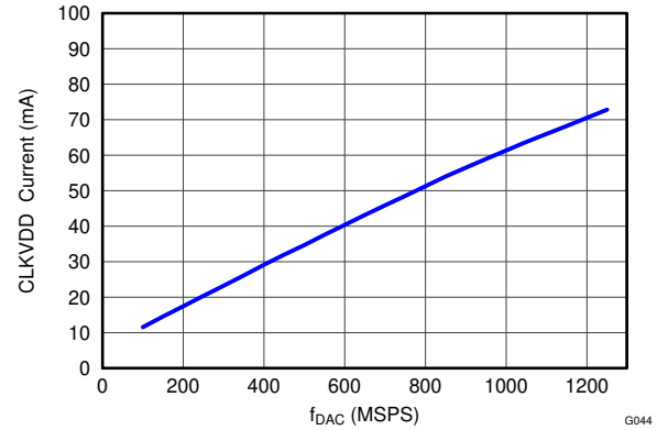
图 5-44. CLKVDD Current vs f_{DAC}
