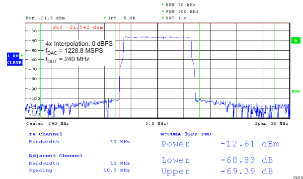
图 5-34. 10 MHz Single Carrier LTE Test Model 3.1
