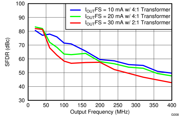
图 5-8. SFDR vs Output Frequency Over I_{OUTFS}
