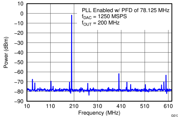
图 5-13. Single Tone Spectral Plot
