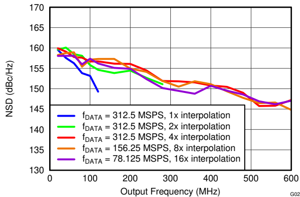
图 5-21. NSD vs Output Frequency Over Interpolation
