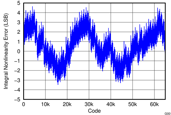
图 5-1. Integral Nonlinearity
