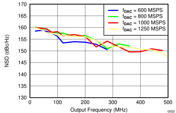
图 5-22. NSD vs Output Frequency Over f_{DAC}
