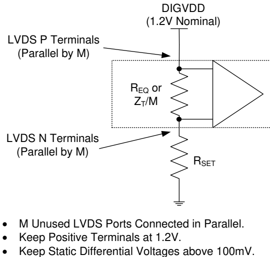
图 6-35. Unused LVDS Ports Connected to Static Logic High Differential Voltage
