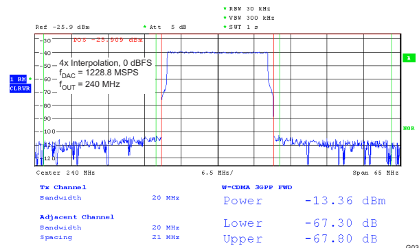
图 5-36. 20 MHz Single Carrier LTE Test Model 3.1
