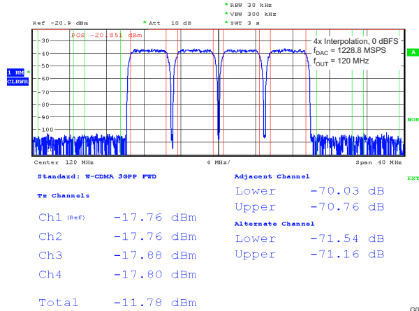
图 5-31. Four Carrier W-CDMA Test Model 1
