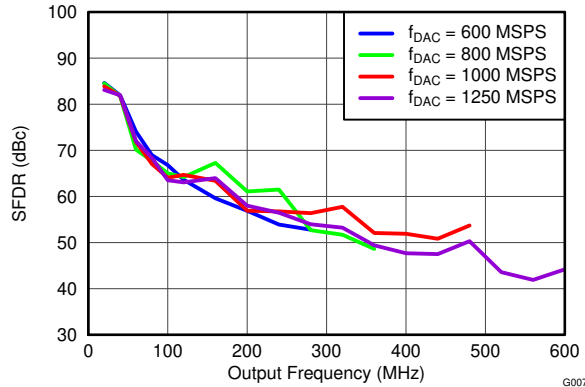
图 5-7. SFDR vs Output Frequency Over f_{DAC}
