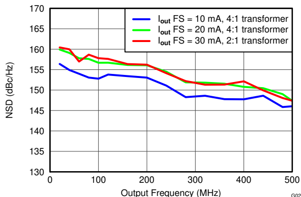
图 5-23. NSD vs Output Frequency Over I_{OUTFS}
