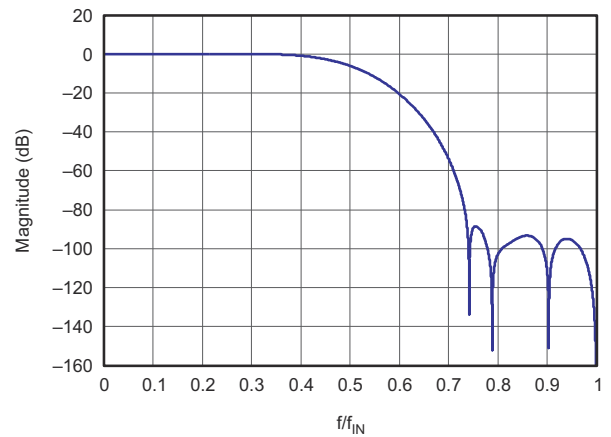
图 6-13. Magnitude Spectrum for FIR1
