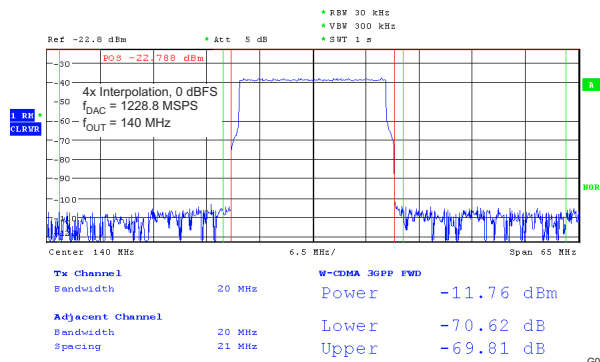
图 5-35. 20 MHz Single Carrier LTE Test Model 3.1
