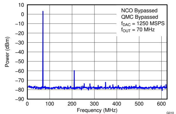
图 5-10. Single Tone Spectral Plot
