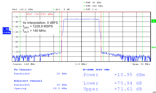
图 5-33. 10 MHz Single Carrier LTE Test Model 3.1
