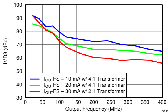
图 5-17. IMD3 vs Output Frequency Over I_{OUTFS}
