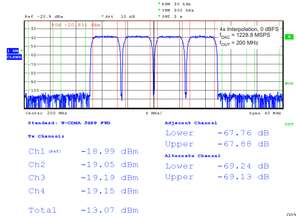
图 5-32. Four Carrier W-CDMA Test Model 1
