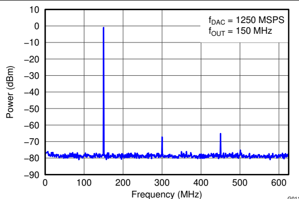
图 5-11. Single Tone Spectral Plot
