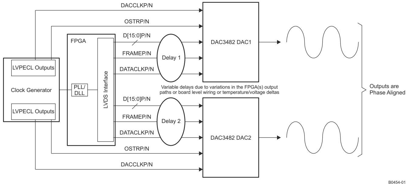
图 6-39. Synchronization System in Dual Sync Sources Mode with PLL Bypassed
