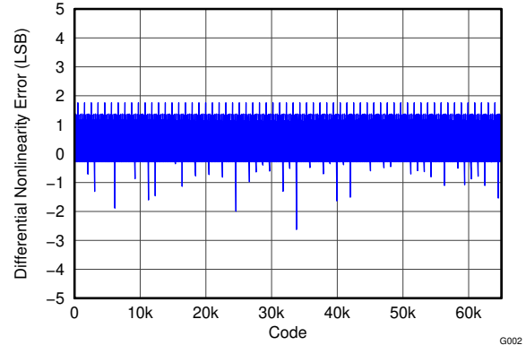
图 5-2. Differential Nonlinearity
