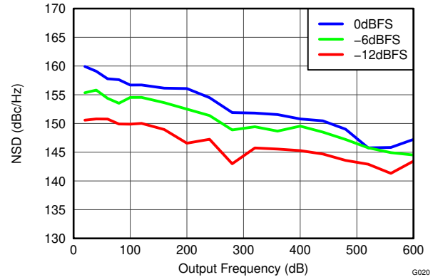
图 5-20. NSD vs Output Frequency Over Input Scale
