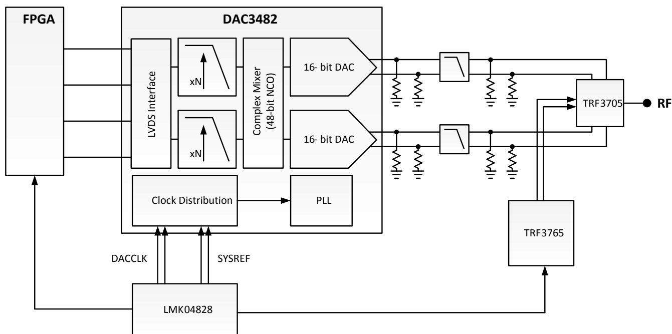
图 7-1. Dual Low-IF Wideband LTE Transmitter Diagram
