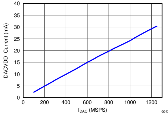
图 5-43. DACVDD Current vs f_{DAC}
