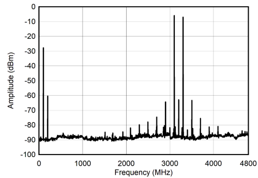
图 6-20. Dual Channel RF Mode: Single Tone Spectrum at 3.1 GHz
