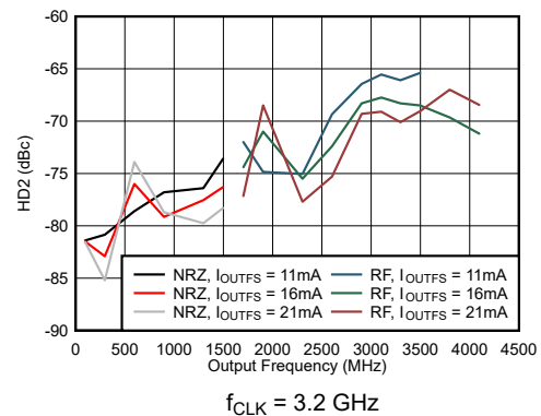
图 6-66. Dual Channel NRZ and RF Mode: HD2 vs Output Frequency and Output Current
