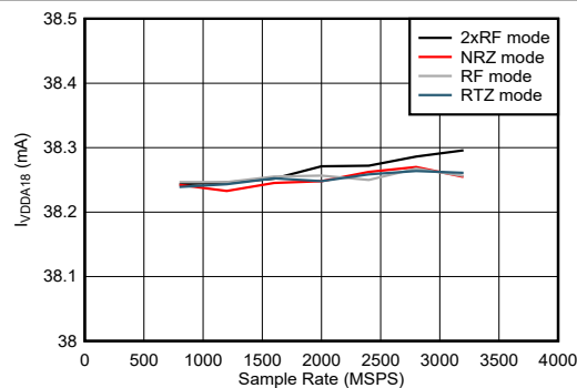
图 6-126. Dual Channel Mode: I_{VDDA18} vs Sample Rate
