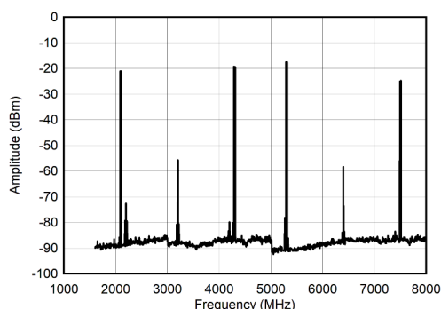
图 6-37. Dual Channel 2xRF Mode: Dual Tone Spectrum at 3.3 to 6.3 GHz \pm 10 MHz
