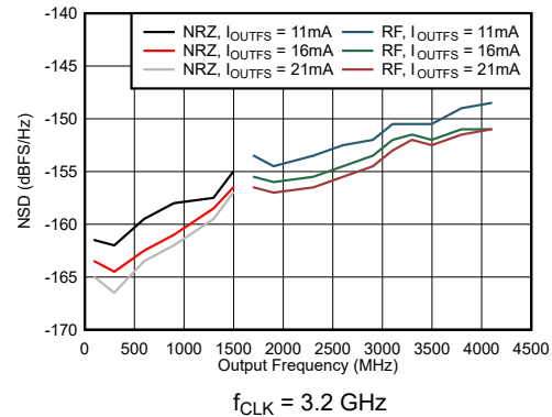
图 6-68. Dual Channel NRZ and RF Mode: NSD vs Output Frequency and Output Current
