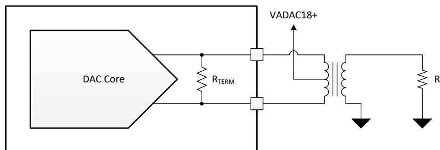
图 7-10. DAC Output Interface using Center-Tapped Transformer
