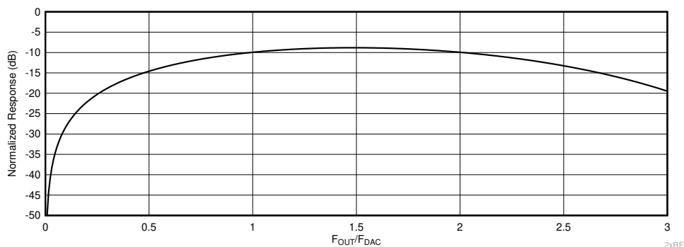
图 7-8. 2xRF Mode Output Waveform Frequency Response
