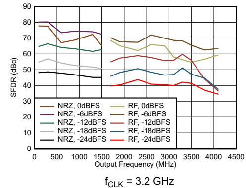
图 6-70. Dual Channel NRZ and RF Mode: SFDR vs Output Frequency and Digital Level
