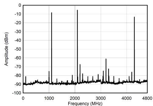
图 6-18. Dual Channel RF Mode: Single Tone Spectrum at 2.1 GHz
