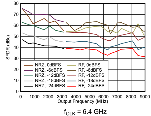
图 6-100. Single Channel NRZ and RF Modes: SFDR vs Output Frequency and Digital Level
