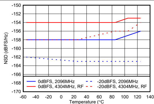
图 6-124. Single Channel Mode: NSD vs Temperature
