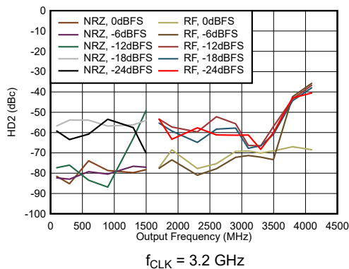
图 6-71. Dual Channel NRZ and RF Mode: HD2 vs Output Frequency and Digital Level
