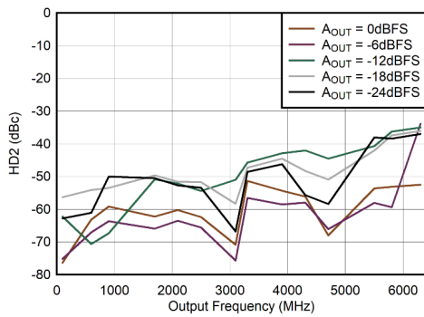
图 6-111. Single Channel RTZ Mode: HD2 vs Output Frequency and Digital Level
