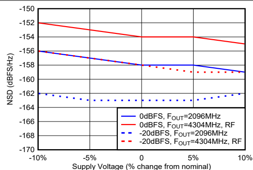
图 6-122. Single Channel Mode: NSD vs Supply Voltage
