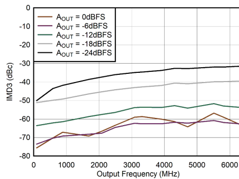
图 6-114. Single Channel RTZ Mode: IMD3 vs Output Frequency and Digital Level
