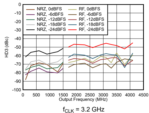
图 6-72. Dual Channel NRZ and RF Mode: HD3 vs Output Frequency and Digital Level
