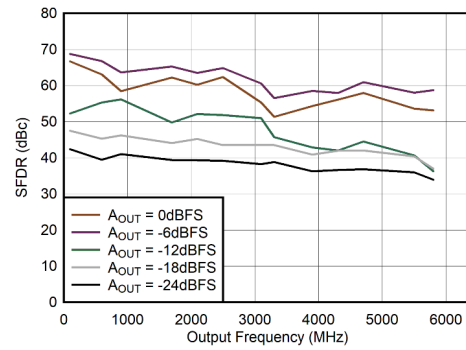
图 6-110. Single Channel RTZ Mode: SFDR vs Output Frequency and Digital Level
