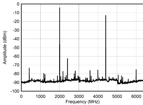
图 6-43. Single Channel NRZ Mode: Single Tone Spectrum at 2 GHz
