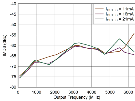
图 6-109. Single Channel RTZ Mode: IMD3 vs Output Frequency and Output Current
