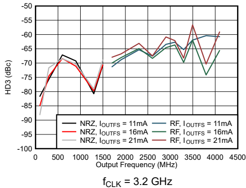
图 6-67. Dual Channel NRZ and RF Mode: HD3 vs Output Frequency and Output Current
