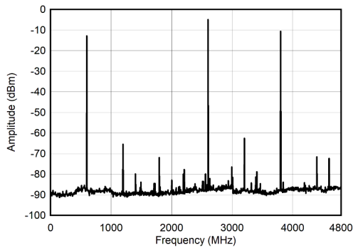
图 6-19. Dual Channel RF Mode: Single Tone Spectrum at 2.6 GHz
