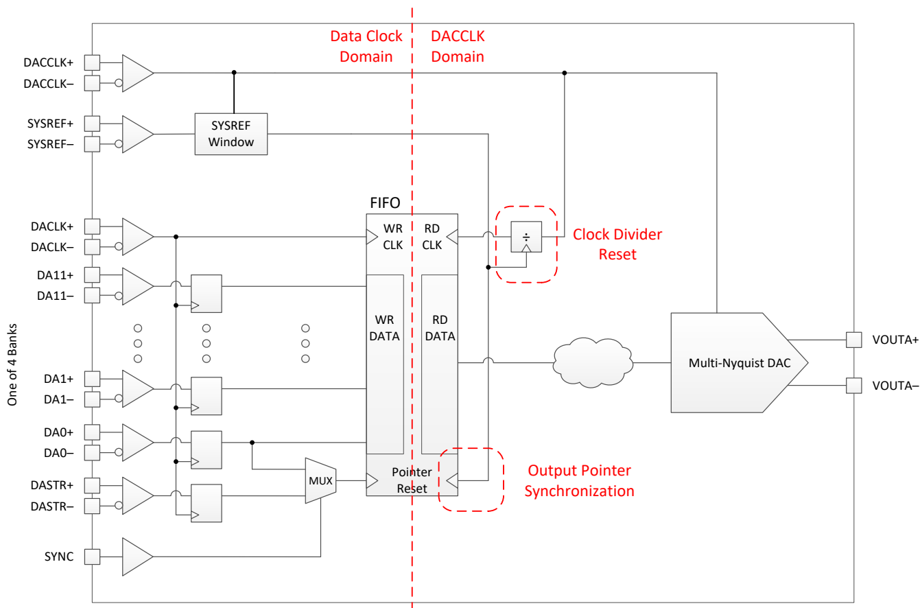
图 7-21. FIFO Synchronization Logic Diagram
