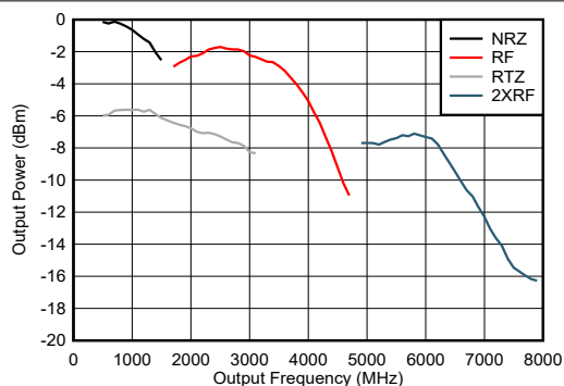
图 6-7. Dual Channel Modes: DAC12DL3200EVM Output Power vs Output Frequency
