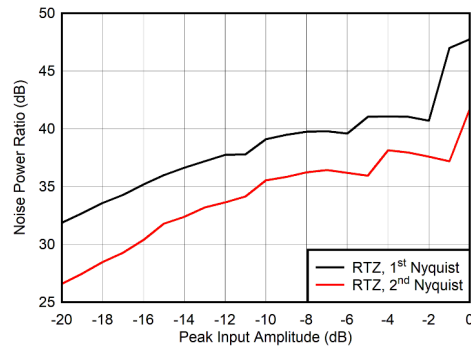
图 6-116. Dual Channel RTZ Mode: NPR vs Digital Level
