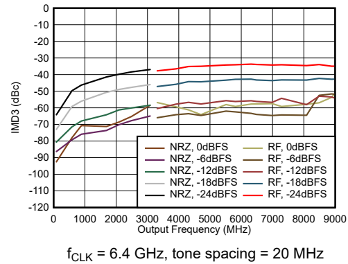
图 6-104. Single Channel NRZ and RF Modes: IMD3 vs Output Frequency and Digital Level
