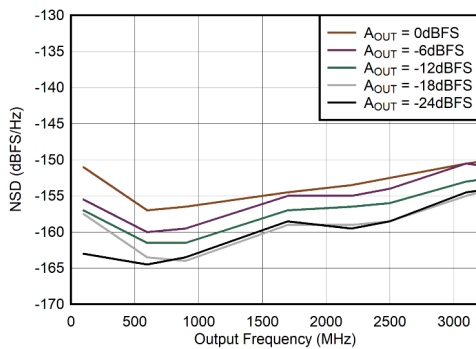
图 6-113. Single Channel RTZ Mode: NSD vs Output Frequency and Digital Level
