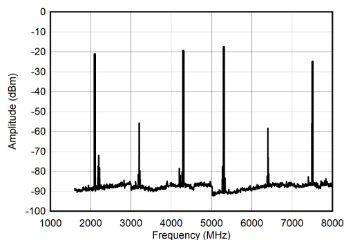
图 6-38. Dual Channel 2xRF Mode: Dual Tone Spectrum at 3.8 to 5.8 GHz \pm 10 MHz
