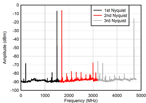
图 6-17. Dual Channel RF Mode: Single Tone Spectrum at 1.7 GHz
