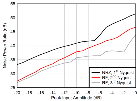
图 6-115. Dual Channel NRZ and RF Modes: NPR vs Digital Level
