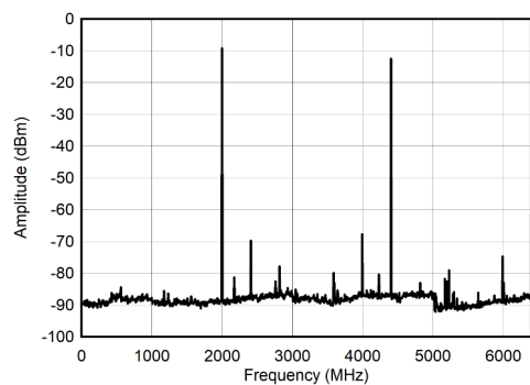
图 6-59. Single Channel RTZ Mode: Single Tone Spectrum at 2 GHz
