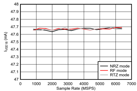
图 6-142. Single Channel Mode: I_{VEE} vs Sample Rate
