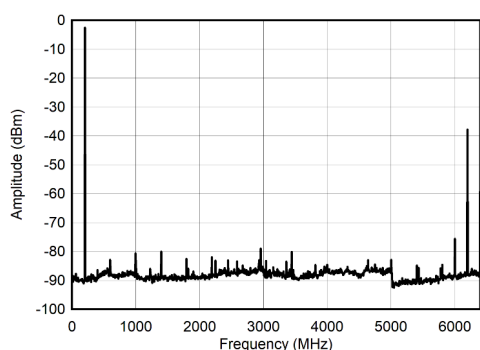
图 6-41. Single Channel NRZ Mode: Single Tone Spectrum at 200 MHz
