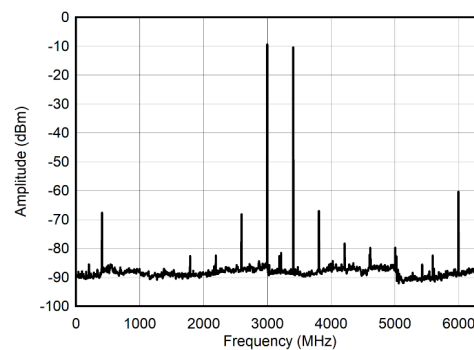
图 6-60. Single Channel RTZ Mode: Single Tone Spectrum at 3 GHz
