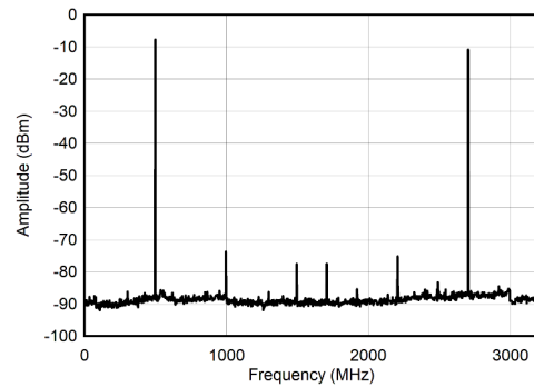
图 6-26. Dual Channel RTZ Mode: Single Tone Spectrum at 500 MHz
