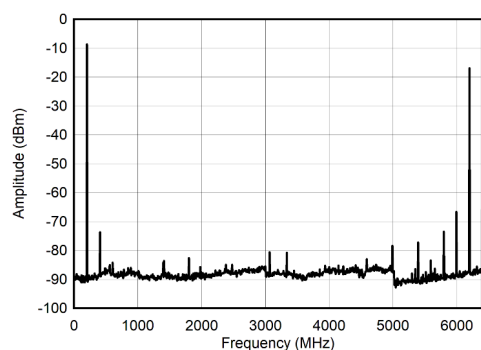
图 6-57. Single Channel RTZ Mode: Single Tone Spectrum at 200 MHz
