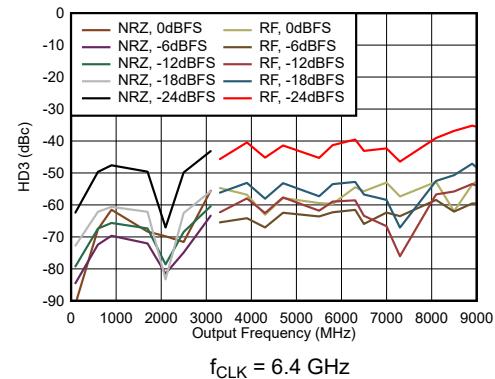
图 6-102. Single Channel NRZ and RF Modes: HD3 vs Output Frequency and Digital Level
