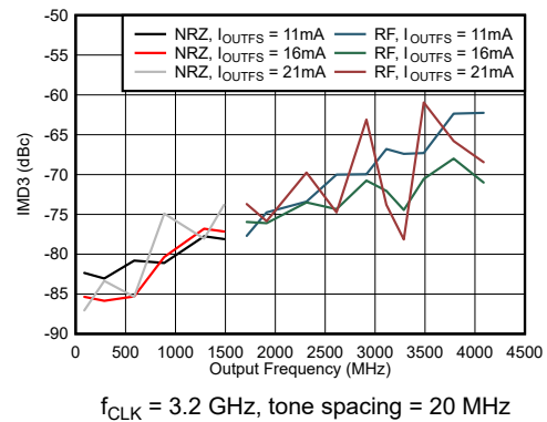
图 6-69. Dual Channel NRZ and RF Mode: IMD3 vs Output Frequency and Output Current
