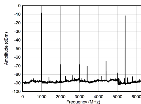
图 6-58. Single Channel RTZ Mode: Single Tone Spectrum at 1 GHz
