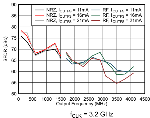
图 6-65. Dual Channel NRZ and RF Mode: SFDR vs Output Frequency and Output Current
