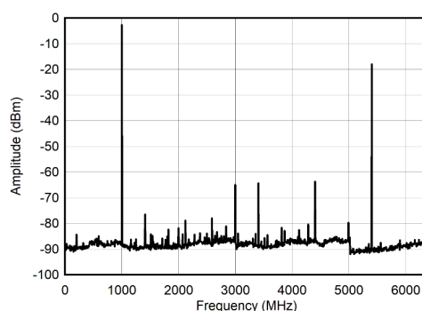
图 6-42. Single Channel NRZ Mode: Single Tone Spectrum at 1 GHz
