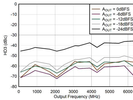
图 6-112. Single Channel RTZ Mode: HD3 vs Output Frequency and Digital Level
