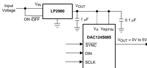
Figure 40. LP2980 Regulator
