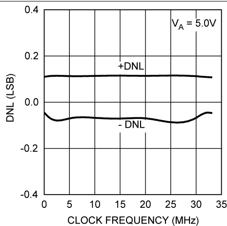
Figure 12. 5-V DNL vs. f_{\text{SCLK}}
