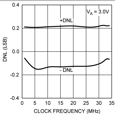
Figure 11. 3-V DNL vs. f_{\text{SCLK}}
