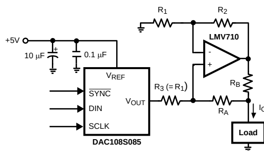
Figure 37. Variable Current Source
