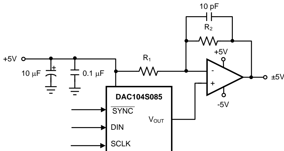
Figure 27. Bipolar Operation
