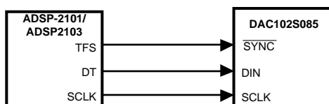
Figure 33. ADSP-2101 and ADSP-2103 Interface
