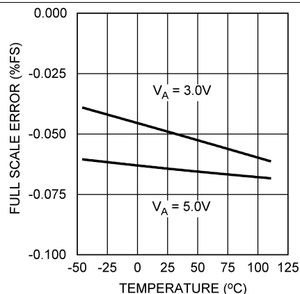
Figure 28. Full-Scale Error vs. Temperature
