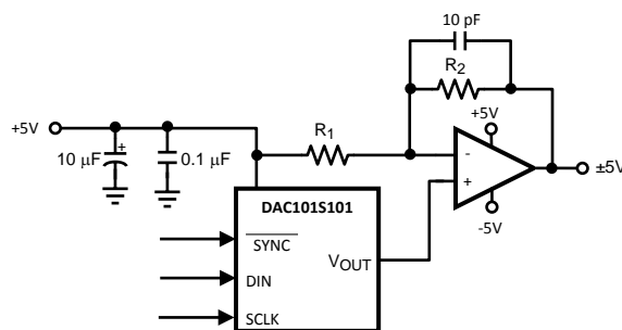
Figure 41. Bipolar Operation
