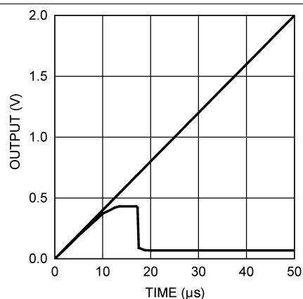
Figure 32. Power-On Reset
