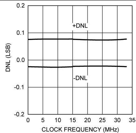
Figure 12. 5-V DNL vs. f_{SCLK}
