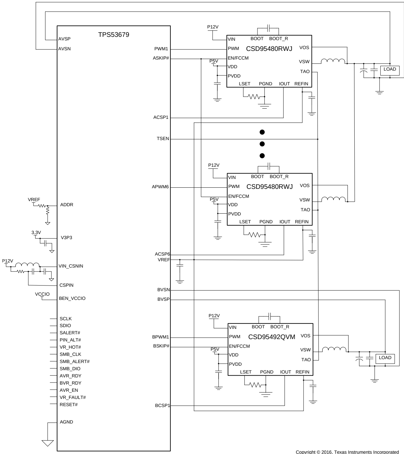
Figure 1. Application Schematic
