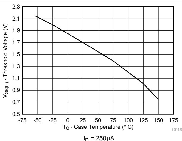
图 4-12. Threshold Voltage vs Temperature
