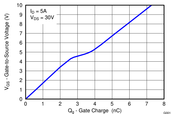
栅极电荷
