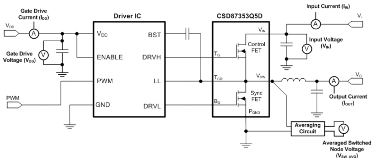
Figure 32. Typical Application
