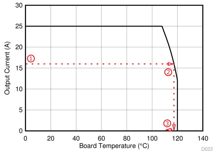
Figure 32. Power Block SOA
