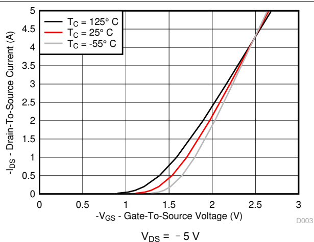
图 5-2. Transfer Characteristics
