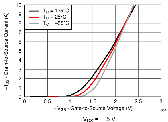
图 5-3. Transfer Characteristics
