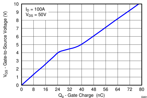
栅极电荷
