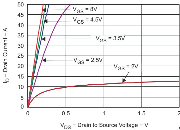
图 7-2. Saturation Characteristics
