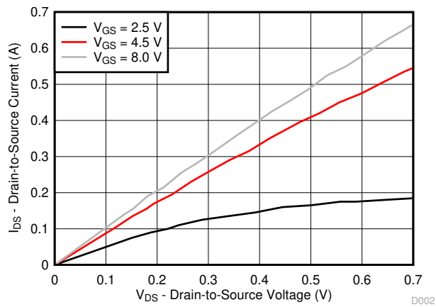
图 5-1. Saturation Characteristics
