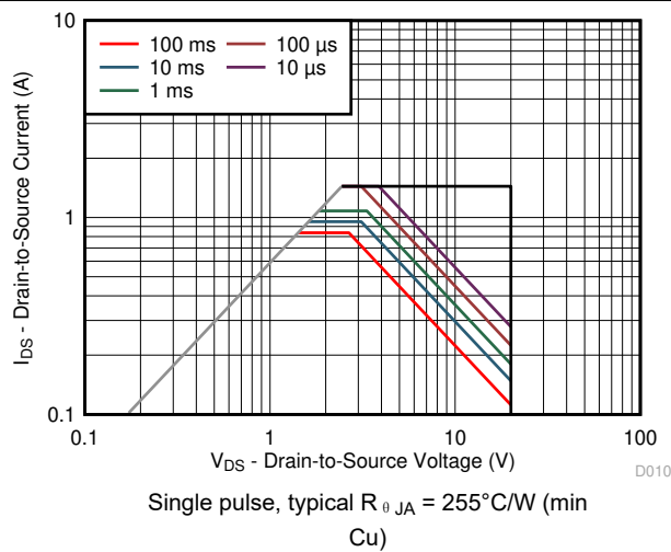
图 5-10. Maximum Safe Operating Area
