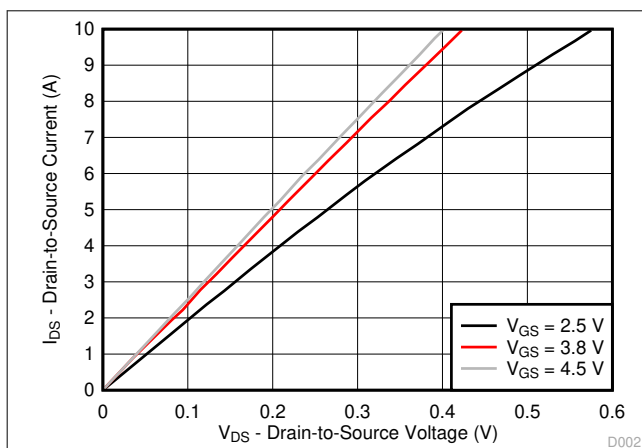
图 5-2. Saturation Characteristics
