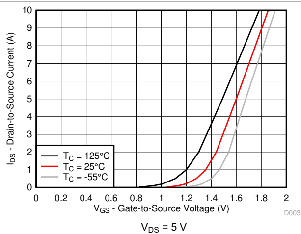
图 5-3. Transfer Characteristics
