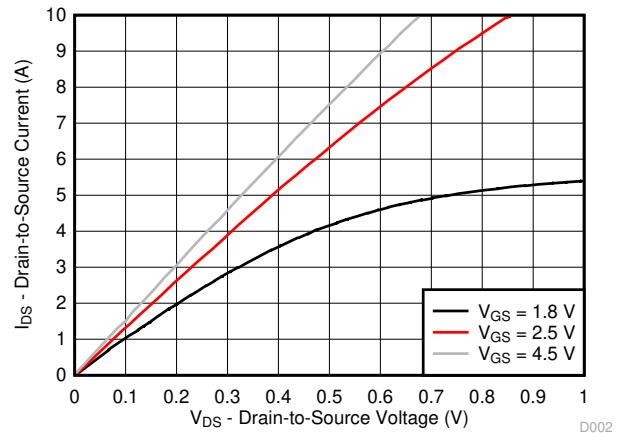
图 5-2. Saturation Characteristics
