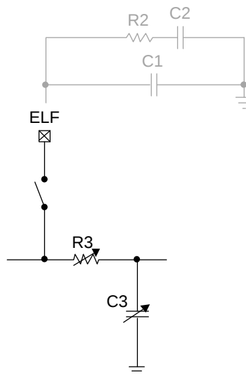
Figure 55. CDCM6208 PLL Loop Filter Topology
