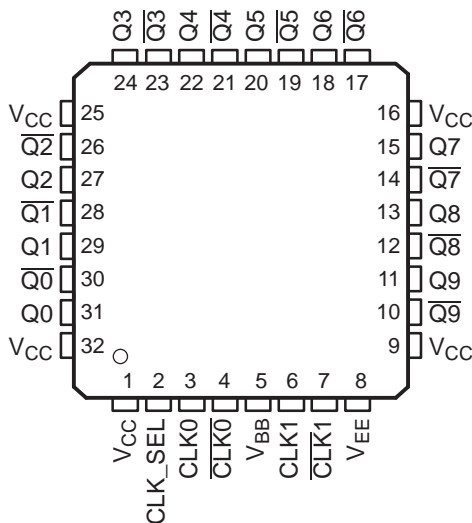
LQFP PACKAGE (TOP VIEW)
