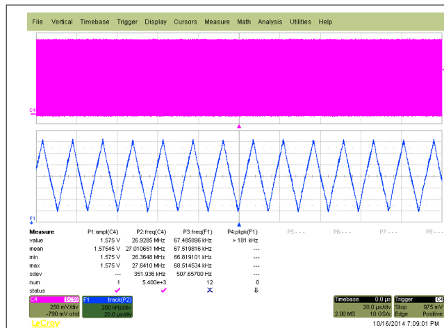
图 9-6. f_{out} = 27\text{MHz} , VCO frequency < 125MHz, SSC (2% center)
