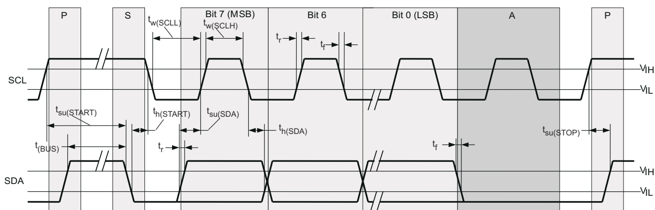
图 7-8. Timing Diagram for SDA/SCL Serial Control Interface
