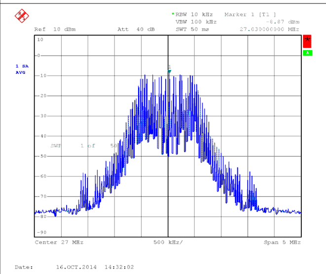
图 8-10. Output Spectrum With SSC On, 2% Center
