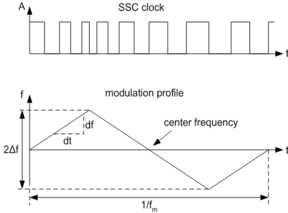
图 8-2. Modulation Frequency ( f_m ) and Modulation Amount
