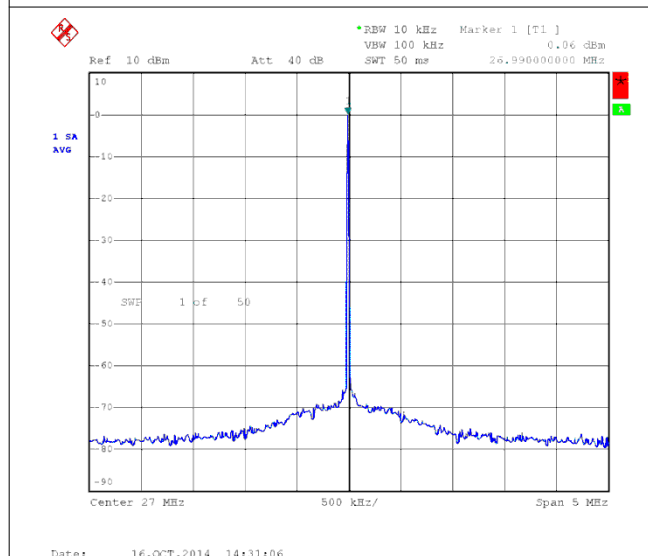
图 8-9. Output Spectrum With SSC Off
