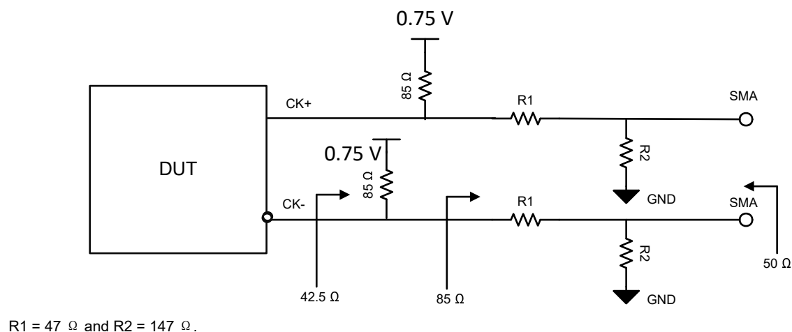
图 7-2. DC Simulation Load (Referencing Intel DB2000QL Document)
