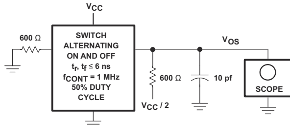
图 14-3. Control-to-Switch Feedthrough Noise Test Circuit
