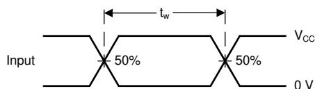
图 5-1. Voltage Waveforms, Standard CMOS Inputs Pulse Duration
