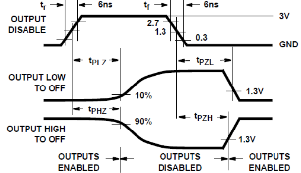
图 6-4. HCT three-state propagation delay waveform
