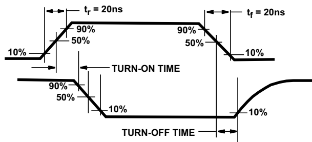
图 6-2. Waveforms, Channel Being Turned ON ( R_L = 1\text{k}\Omega )
