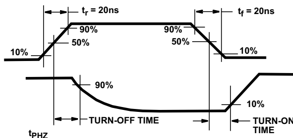
图 6-3. Waveforms, Channel Being Turned OFF ( R_L = 1\text{k}\Omega )
