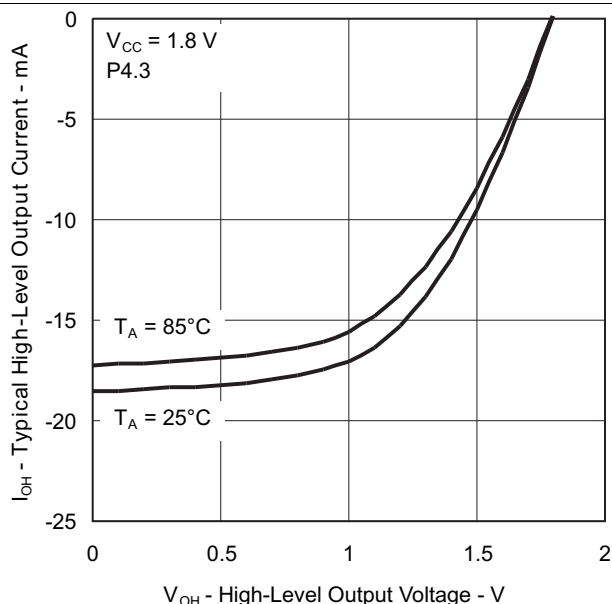
Figure 5-14. Typical High-Level Output Current vs High-Level Output Voltage
